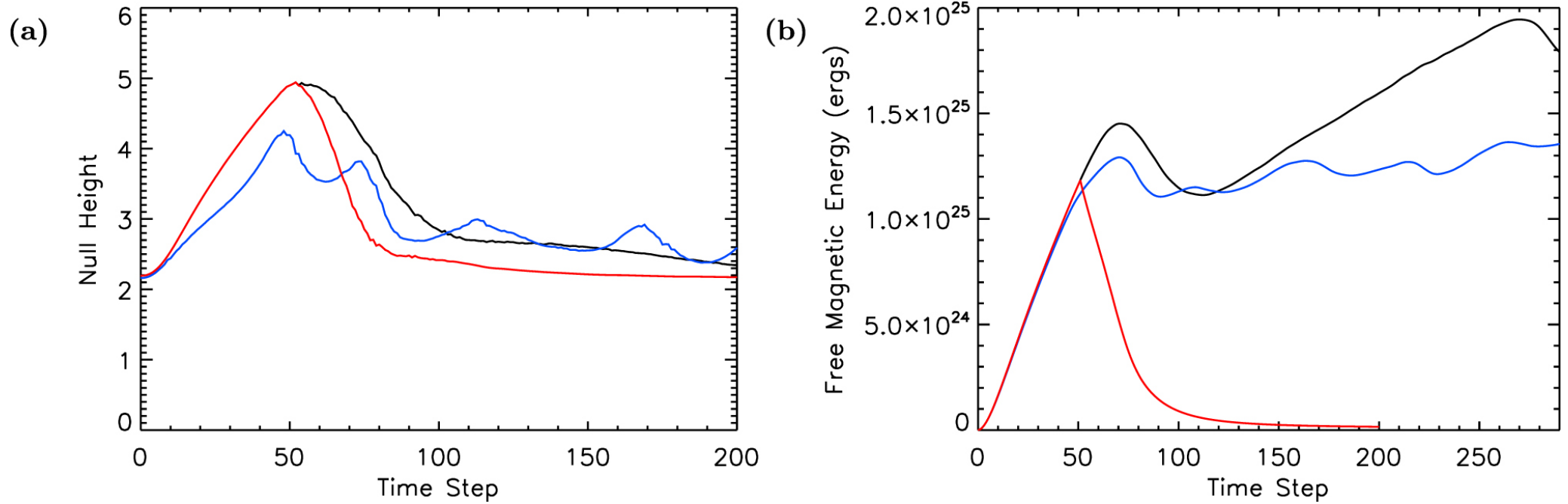
Figure 4. from Nonlinear Force-free Field Modeling of Solar Coronal Jets in Theoretical Configurations null 2019 APJ 880 62 doi:10.3847/1538-4357/ab271a https://dx.doi.org/10.3847/1538-4357/ab271a © 2019. The American Astronomical Society. All rights reserved.
