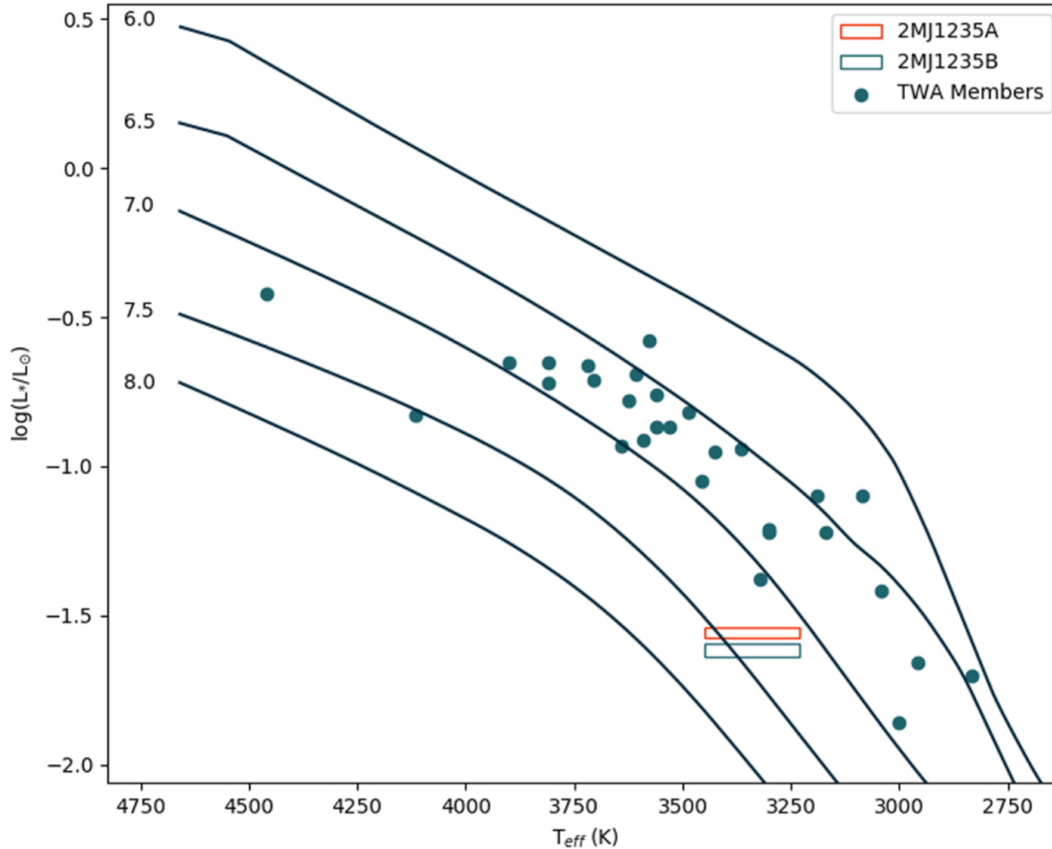
Figure 3. from Radial Velocities of Low-mass Candidate TWA Members null 2019 APJ 879 63 doi:10.3847/1538-4357/ab2591 https://dx.doi.org/10.3847/1538-4357/ab2591 © 2019. The American Astronomical Society. All rights reserved.
