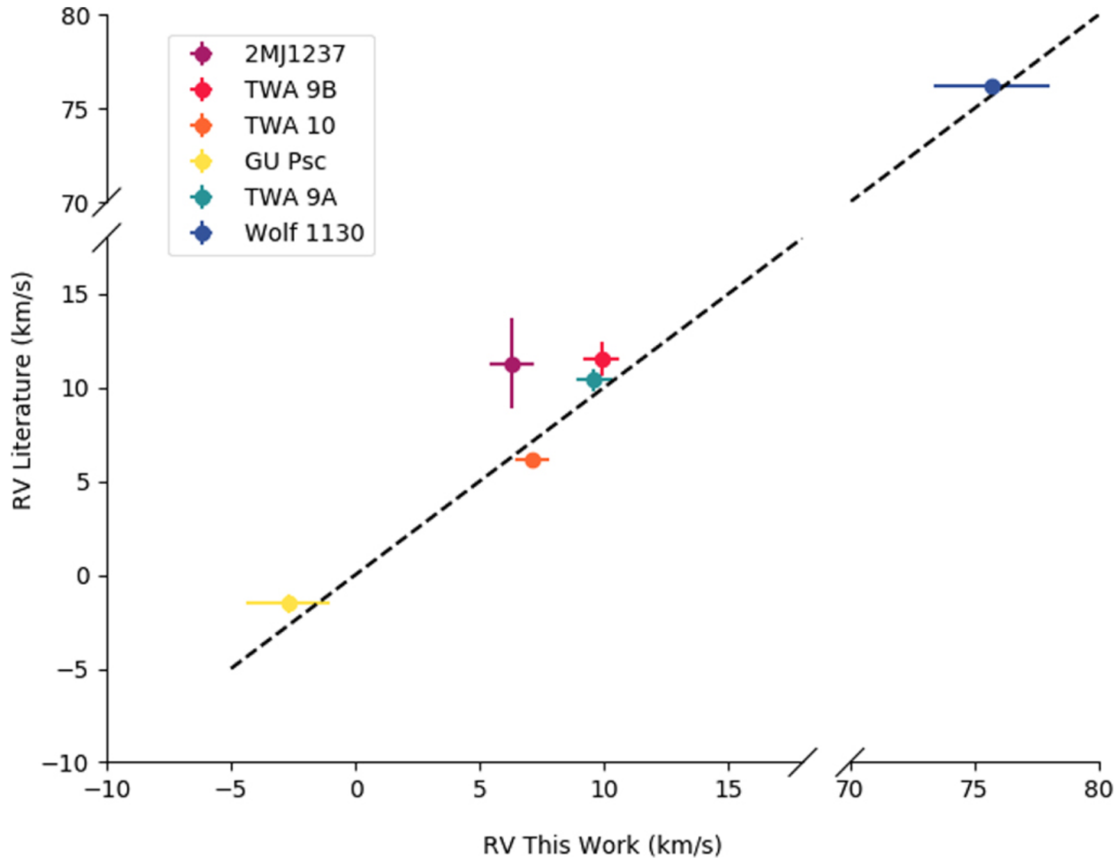
Figure 2. from Radial Velocities of Low-mass Candidate TWA Members null 2019 APJ 879 63 doi:10.3847/1538-4357/ab2591 https://dx.doi.org/10.3847/1538-4357/ab2591 © 2019. The American Astronomical Society. All rights reserved.
