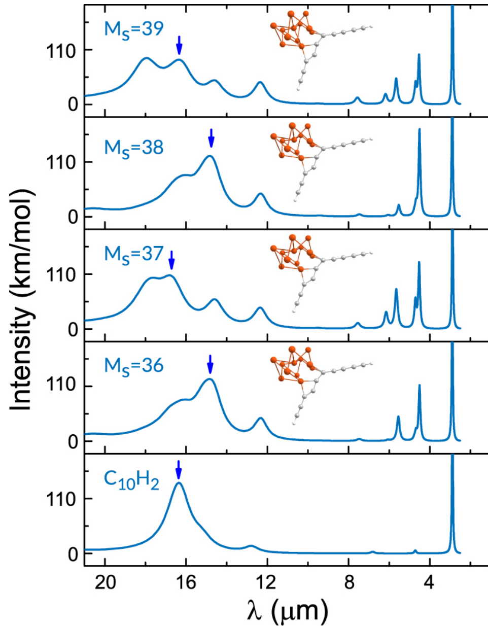
Figure 9. from On the Structure, Magnetic Properties, and Infrared Spectra of Iron Pseudocarbynes in the Interstellar Medium null 2019 APJ 879 2 doi:10.3847/1538-4357/ab22b7 https://dx.doi.org/10.3847/1538-4357/ab22b7 © 2019. The American Astronomical Society. All rights reserved.
