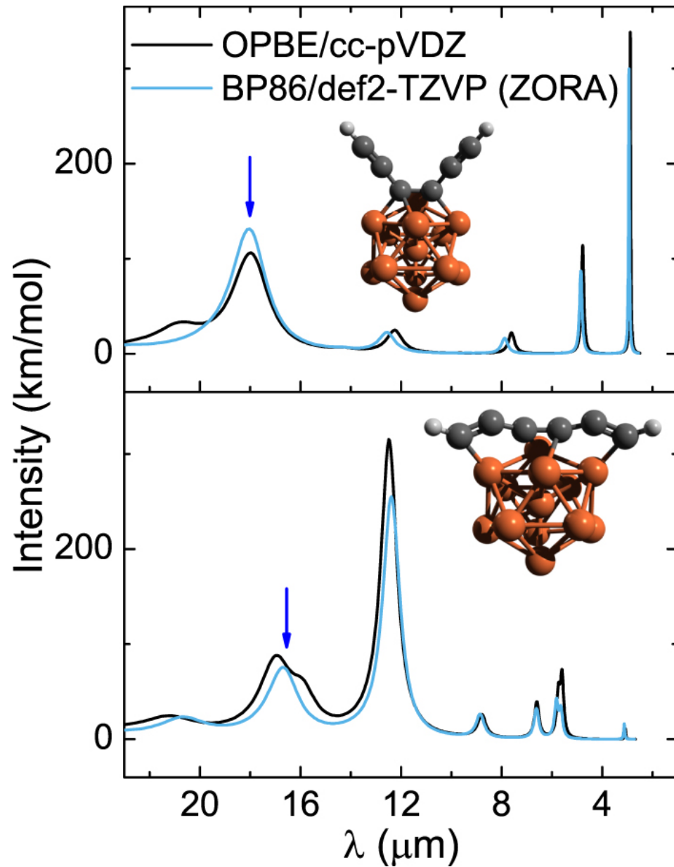
Figure 8. from On the Structure, Magnetic Properties, and Infrared Spectra of Iron Pseudocarbynes in the Interstellar Medium null 2019 APJ 879 2 doi:10.3847/1538-4357/ab22b7 https://dx.doi.org/10.3847/1538-4357/ab22b7 © 2019. The American Astronomical Society. All rights reserved.
