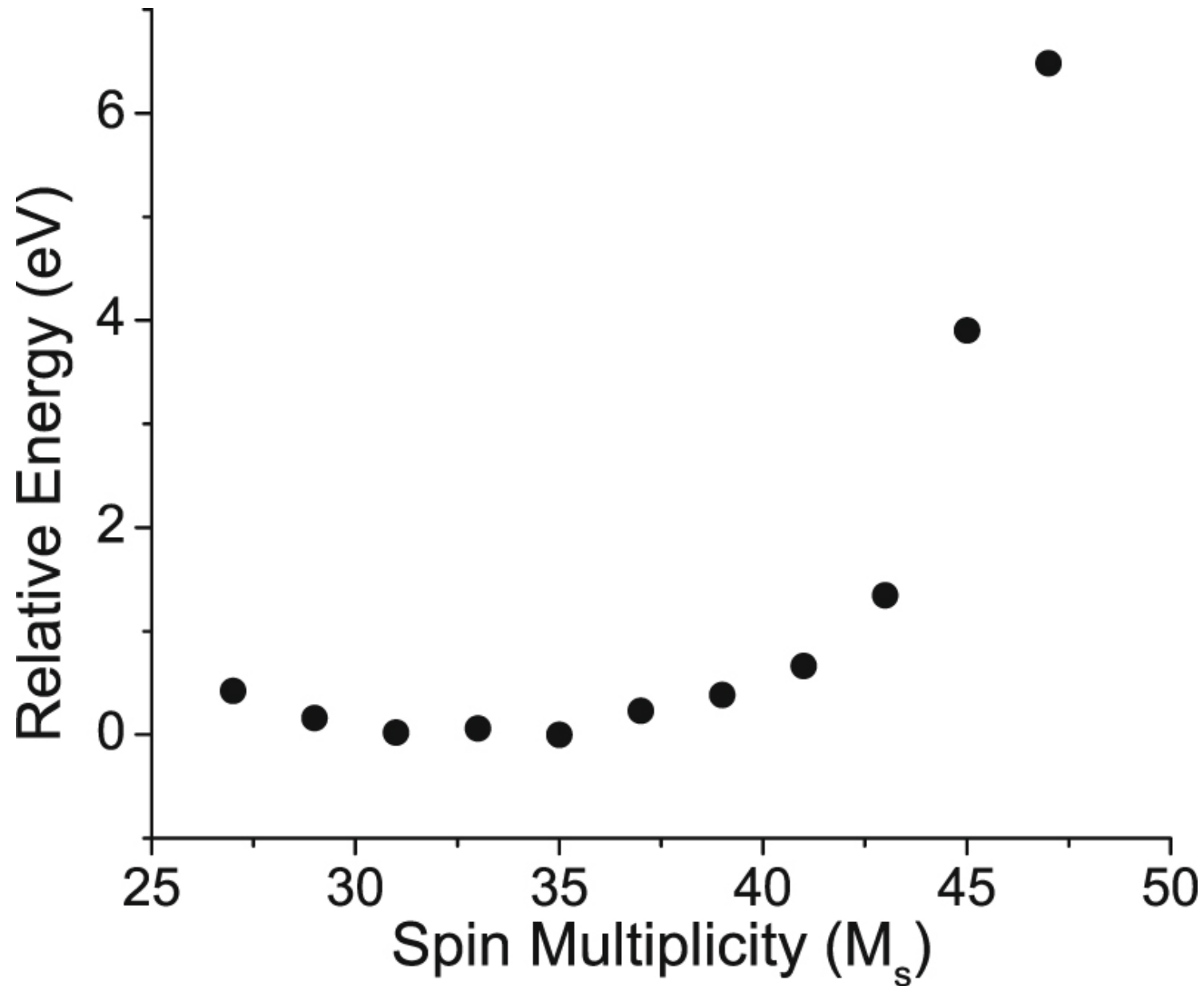
Figure 6. from On the Structure, Magnetic Properties, and Infrared Spectra of Iron Pseudocarbynes in the Interstellar Medium null 2019 APJ 879 2 doi:10.3847/1538-4357/ab22b7 https://dx.doi.org/10.3847/1538-4357/ab22b7 © 2019. The American Astronomical Society. All rights reserved.
