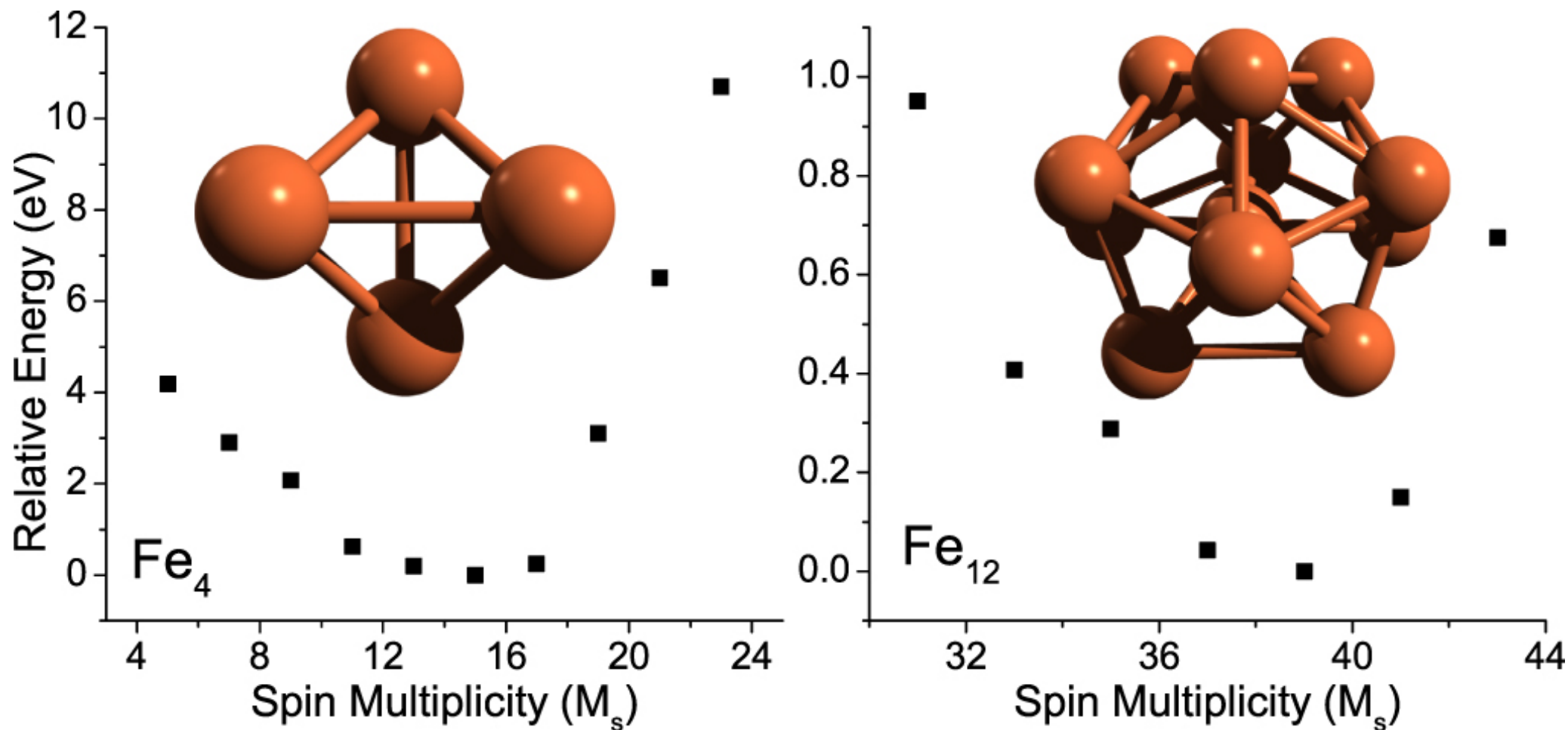
Figure 3. from On the Structure, Magnetic Properties, and Infrared Spectra of Iron Pseudocarbynes in the Interstellar Medium null 2019 APJ 879 2 doi:10.3847/1538-4357/ab22b7 https://dx.doi.org/10.3847/1538-4357/ab22b7
