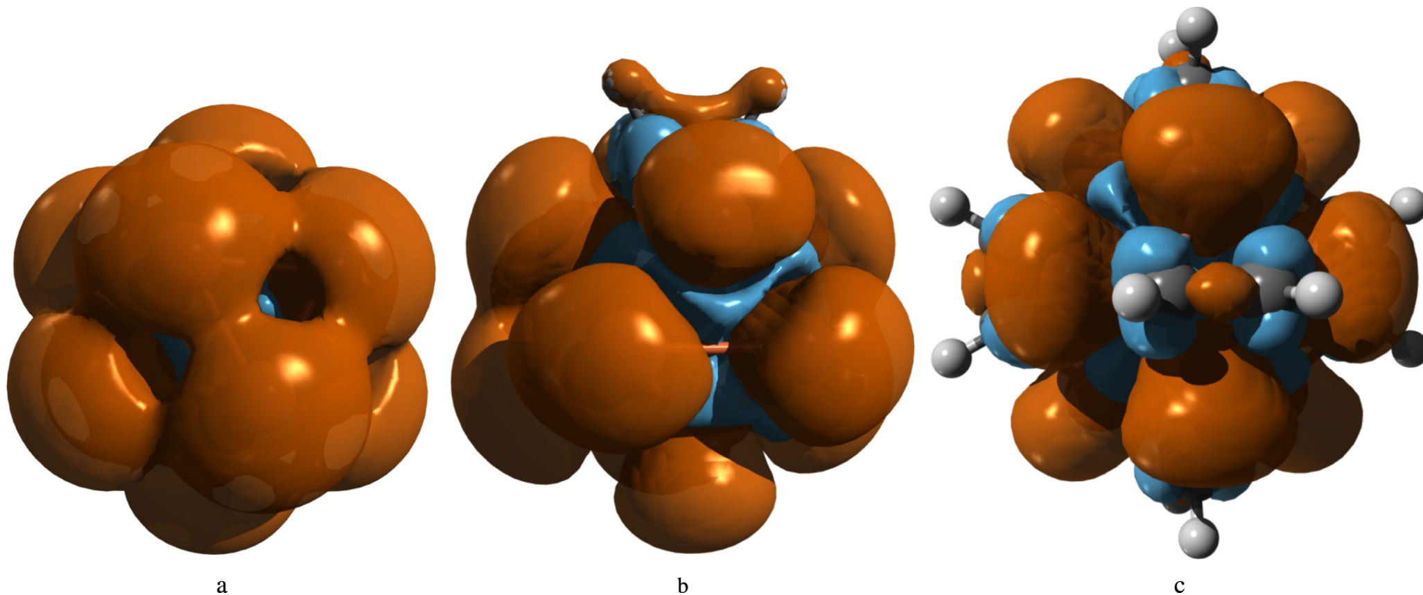
Figure 10. from On the Structure, Magnetic Properties, and Infrared Spectra of Iron Pseudocarbynes in the Interstellar Medium null 2019 APJ 879 2 doi:10.3847/1538-4357/ab22b7 https://dx.doi.org/10.3847/1538-4357/ab22b7 © 2019. The American Astronomical Society. All rights reserved.
