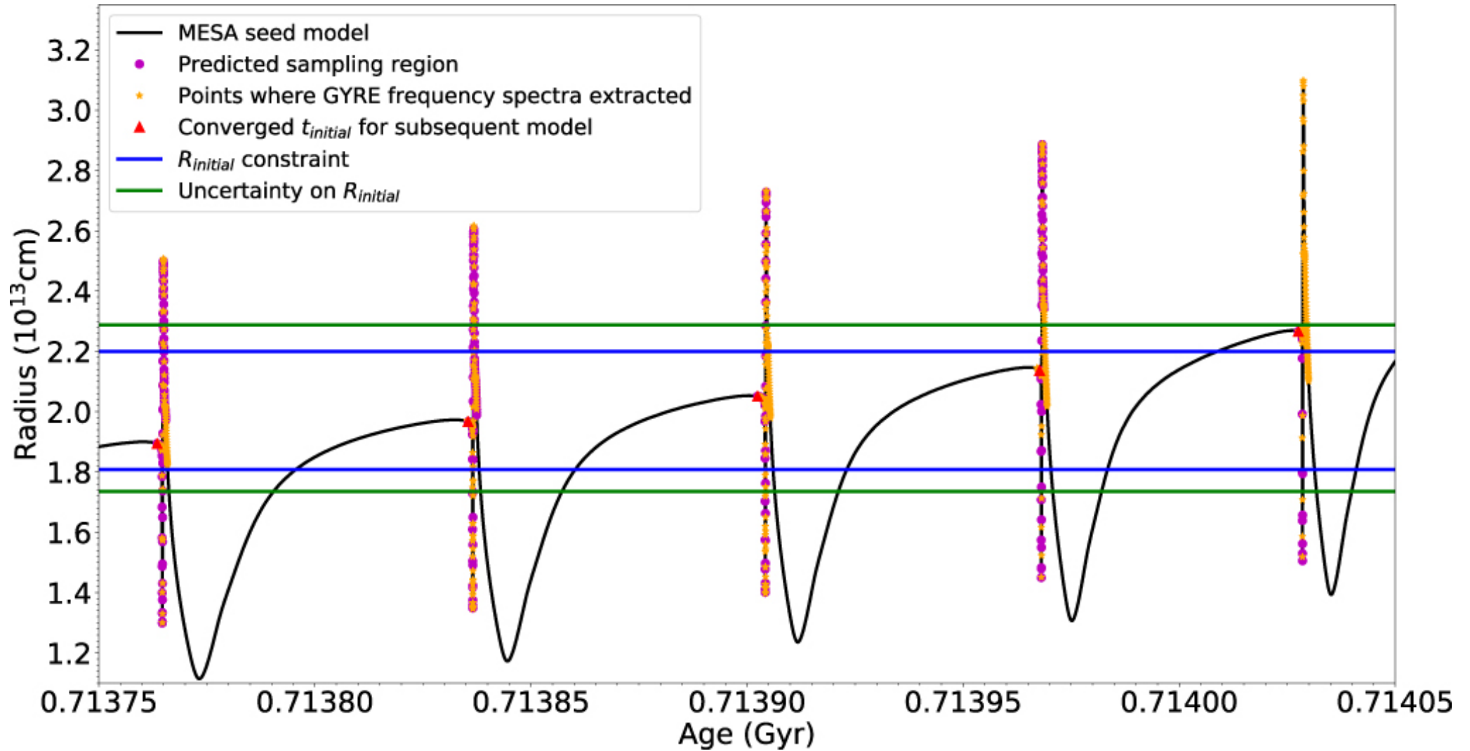
Figure 9. from Stellar Evolution in Real Time: Models Consistent with the Direct Observation of a Thermal Pulse in T Ursae Minoris null 2019 APJ 879 62 doi:10.3847/1538-4357/ab22a5 https://dx.doi.org/10.3847/1538-4357/ab22a5 © 2019. The American Astronomical Society. All rights reserved.
