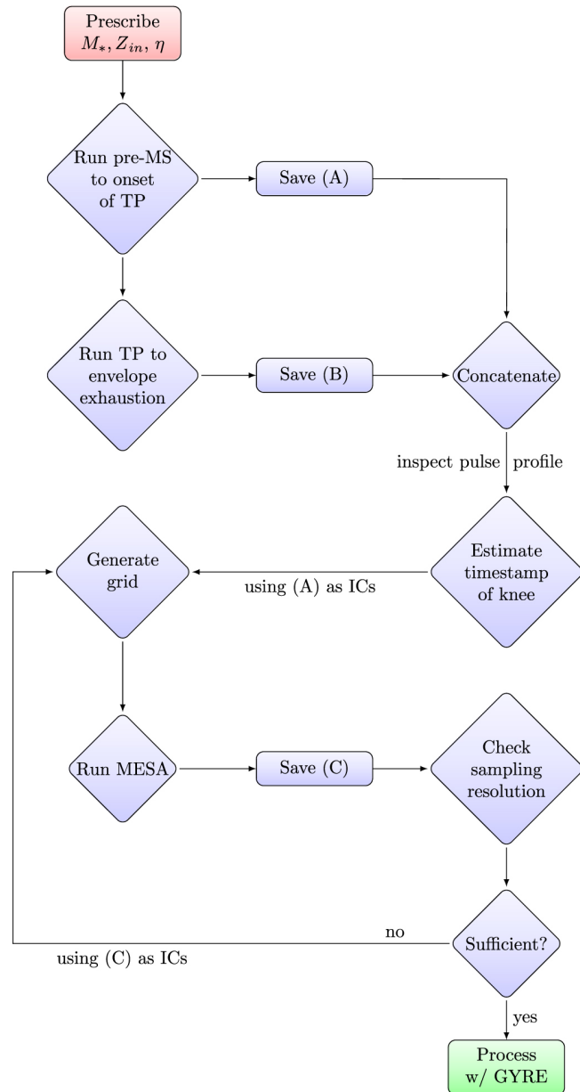
Figure 8. from Stellar Evolution in Real Time: Models Consistent with the Direct Observation of a Thermal Pulse in T Ursae Minoris null 2019 APJ 879 62 doi:10.3847/1538-4357/ab22a5 https://dx.doi.org/10.3847/1538-4357/ab22a5 © 2019. The American Astronomical Society. All rights reserved.
