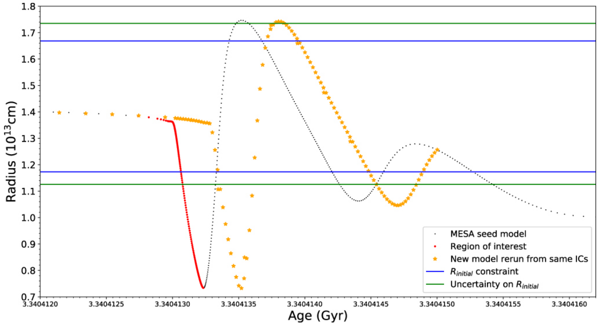
Figure 7. from Stellar Evolution in Real Time: Models Consistent with the Direct Observation of a Thermal Pulse in T Ursae Minoris null 2019 APJ 879 62 doi:10.3847/1538-4357/ab22a5 https://dx.doi.org/10.3847/1538-4357/ab22a5 © 2019. The American Astronomical Society. All rights reserved.
