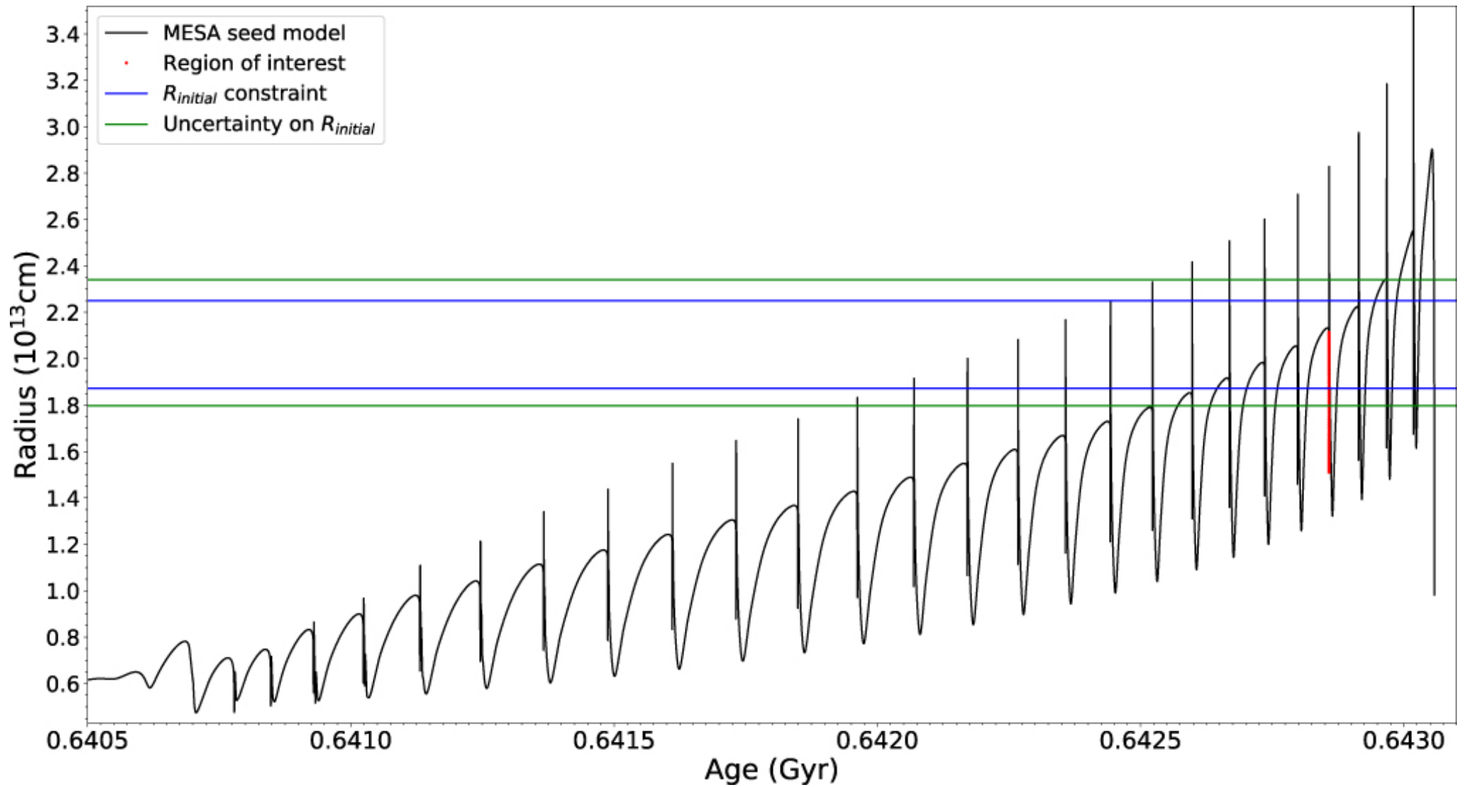
Figure 6. from Stellar Evolution in Real Time: Models Consistent with the Direct Observation of a Thermal Pulse in T Ursae Minoris null 2019 APJ 879 62 doi:10.3847/1538-4357/ab22a5 https://dx.doi.org/10.3847/1538-4357/ab22a5 © 2019. The American Astronomical Society. All rights reserved.
