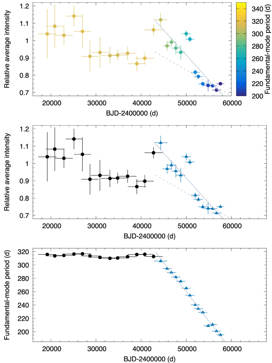
Figure 5. from Stellar Evolution in Real Time: Models Consistent with the Direct Observation of a Thermal Pulse in T Ursae Minoris null 2019 APJ 879 62 doi:10.3847/1538-4357/ab22a5 https://dx.doi.org/10.3847/1538-4357/ab22a5
