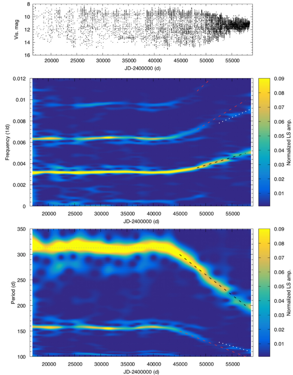
Figure 4. from Stellar Evolution in Real Time: Models Consistent with the Direct Observation of a Thermal Pulse in T Ursae Minoris null 2019 APJ 879 62 doi:10.3847/1538-4357/ab22a5 https://dx.doi.org/10.3847/1538-4357/ab22a5 © 2019. The American Astronomical Society. All rights reserved.
