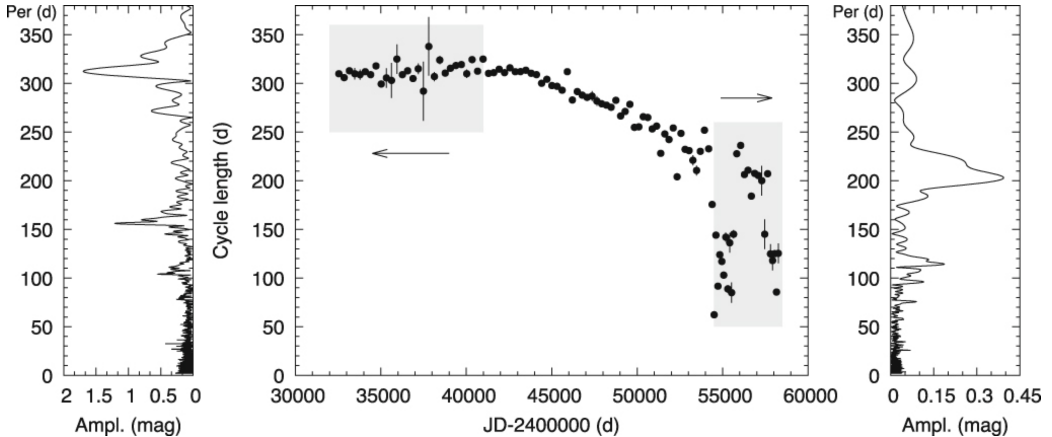
Figure 2. from Stellar Evolution in Real Time: Models Consistent with the Direct Observation of a Thermal Pulse in T Ursae Minoris null 2019 APJ 879 62 doi:10.3847/1538-4357/ab22a5 https://dx.doi.org/10.3847/1538-4357/ab22a5 © 2019. The American Astronomical Society. All rights reserved.
