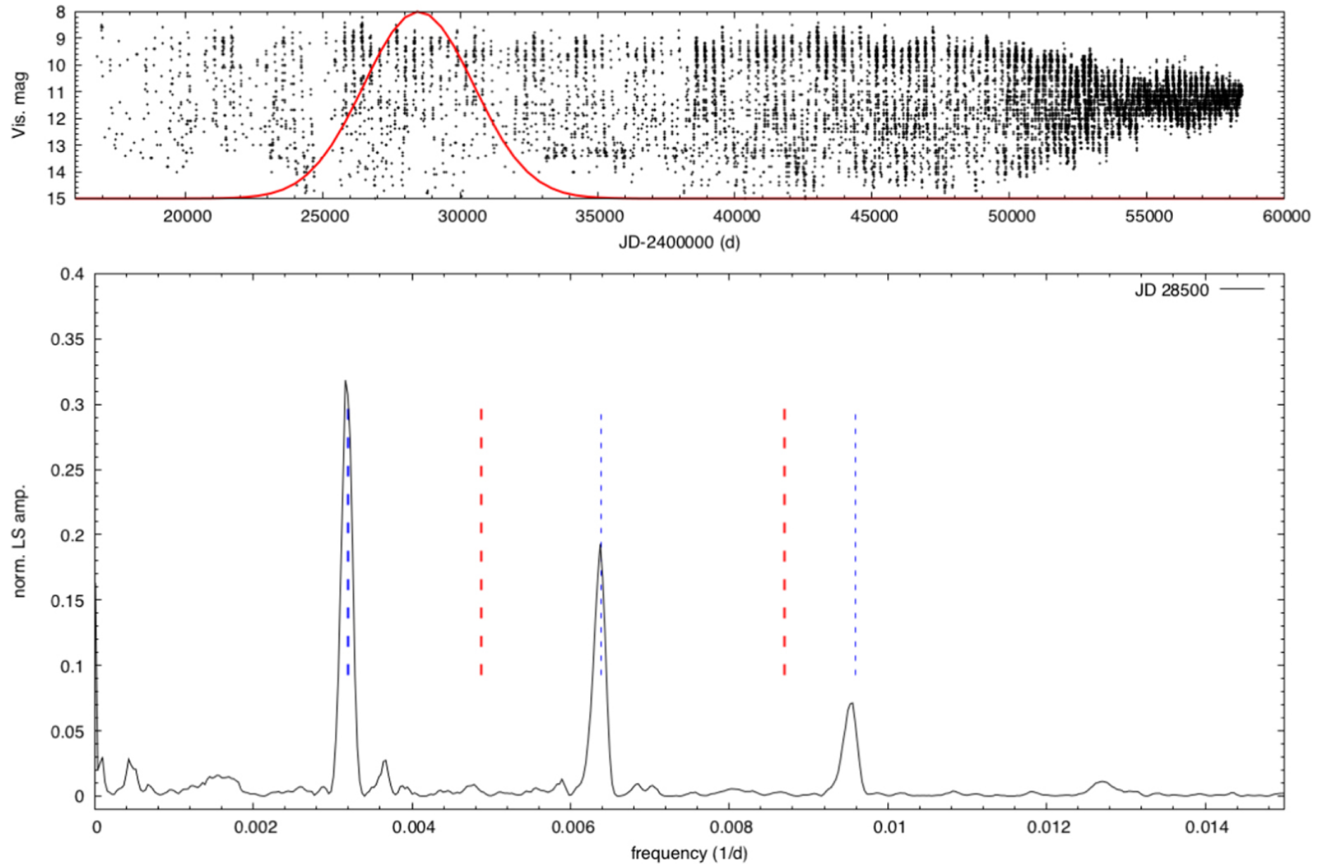
Figure 15. from Stellar Evolution in Real Time: Models Consistent with the Direct Observation of a Thermal Pulse in T Ursae Minoris null 2019 APJ 879 62 doi:10.3847/1538-4357/ab22a5 https://dx.doi.org/10.3847/1538-4357/ab22a5 © 2019. The American Astronomical Society. All rights reserved.
