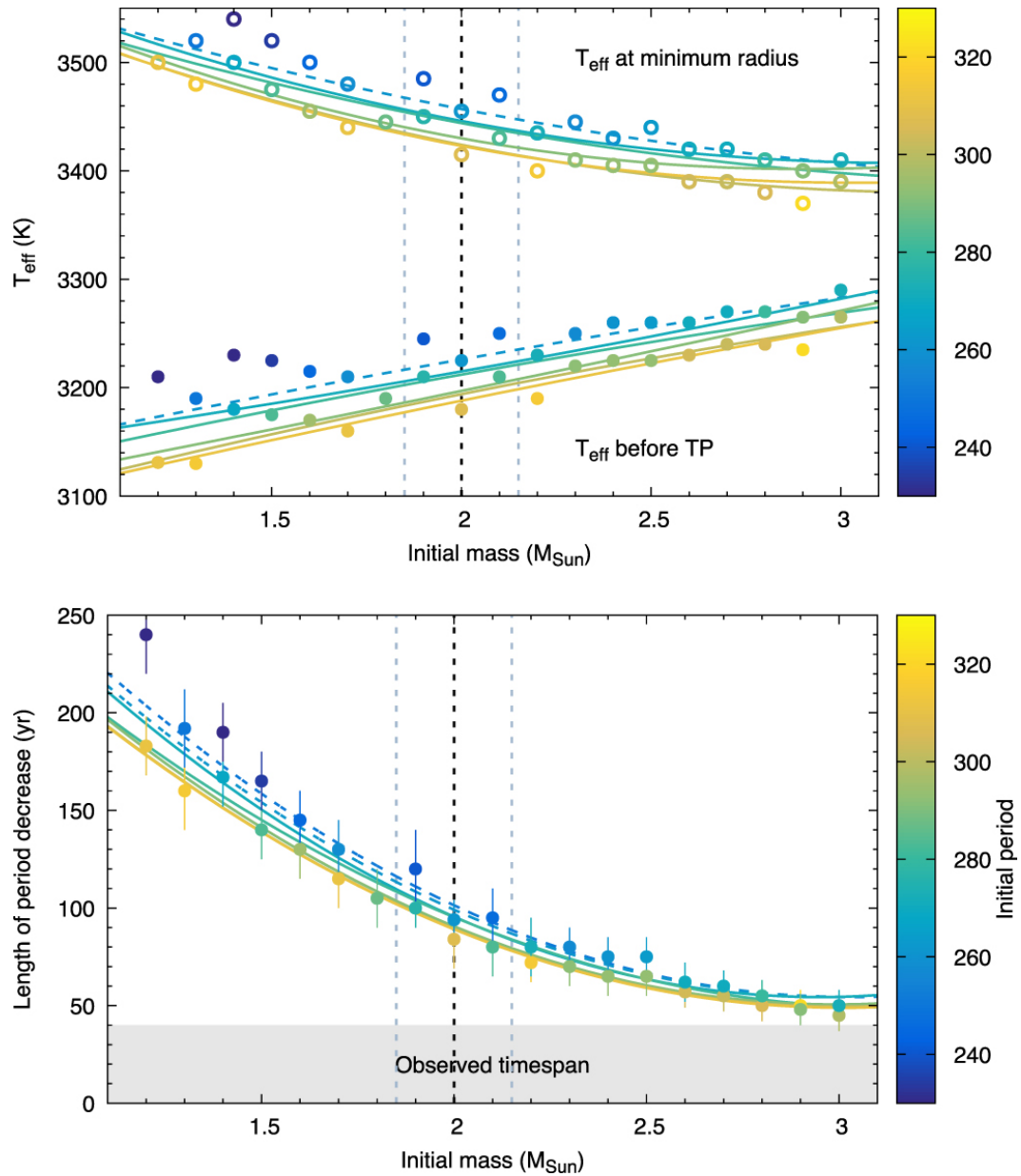
Figure 12. from Stellar Evolution in Real Time: Models Consistent with the Direct Observation of a Thermal Pulse in T Ursae Minoris null 2019 APJ 879 62 doi:10.3847/1538-4357/ab22a5 https://dx.doi.org/10.3847/1538-4357/ab22a5
