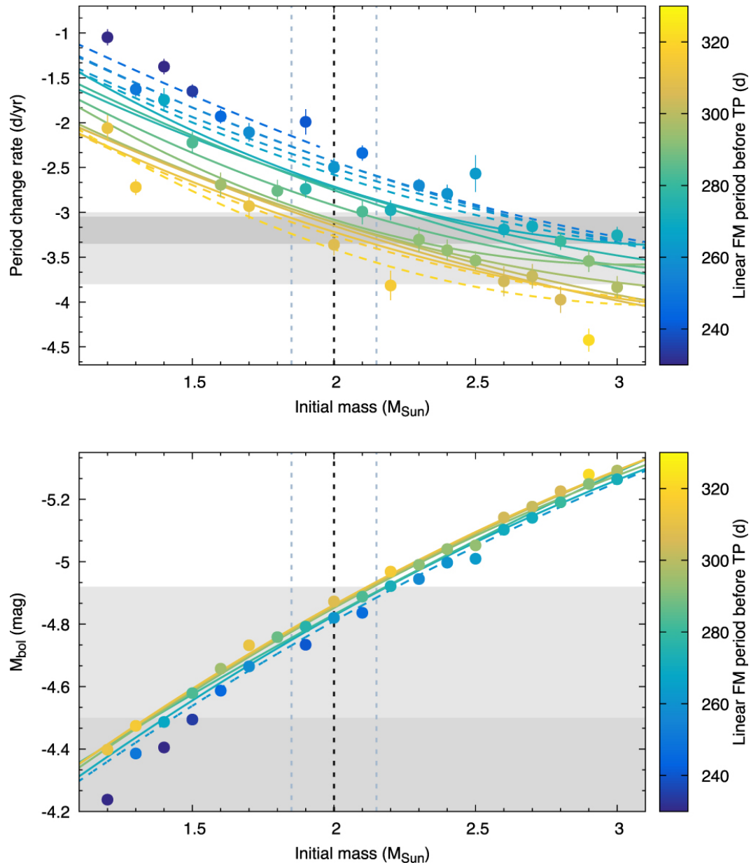
Figure 11. from Stellar Evolution in Real Time: Models Consistent with the Direct Observation of a Thermal Pulse in T Ursae Minoris null 2019 APJ 879 62 doi:10.3847/1538-4357/ab22a5 https://dx.doi.org/10.3847/1538-4357/ab22a5 © 2019. The American Astronomical Society. All rights reserved.
