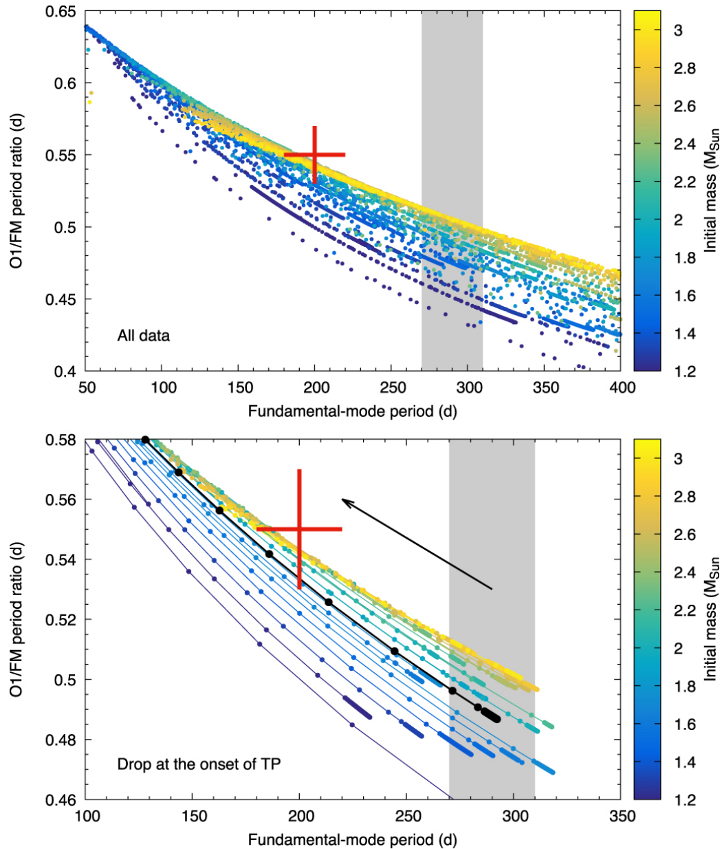
Figure 10. from Stellar Evolution in Real Time: Models Consistent with the Direct Observation of a Thermal Pulse in T Ursae Minoris null 2019 APJ 879 62 doi:10.3847/1538-4357/ab22a5 https://dx.doi.org/10.3847/1538-4357/ab22a5
