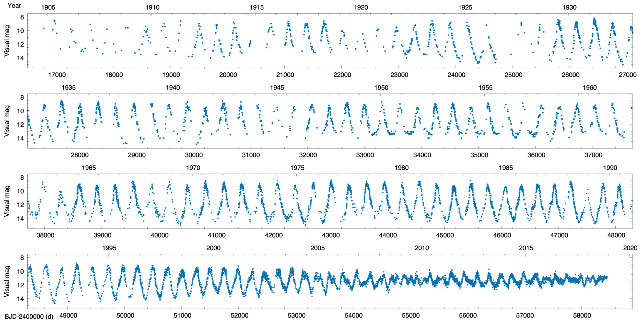
Figure 1. from Stellar Evolution in Real Time: Models Consistent with the Direct Observation of a Thermal Pulse in T Ursae Minoris null 2019 APJ 879 62 doi:10.3847/1538-4357/ab22a5 https://dx.doi.org/10.3847/1538-4357/ab22a5
