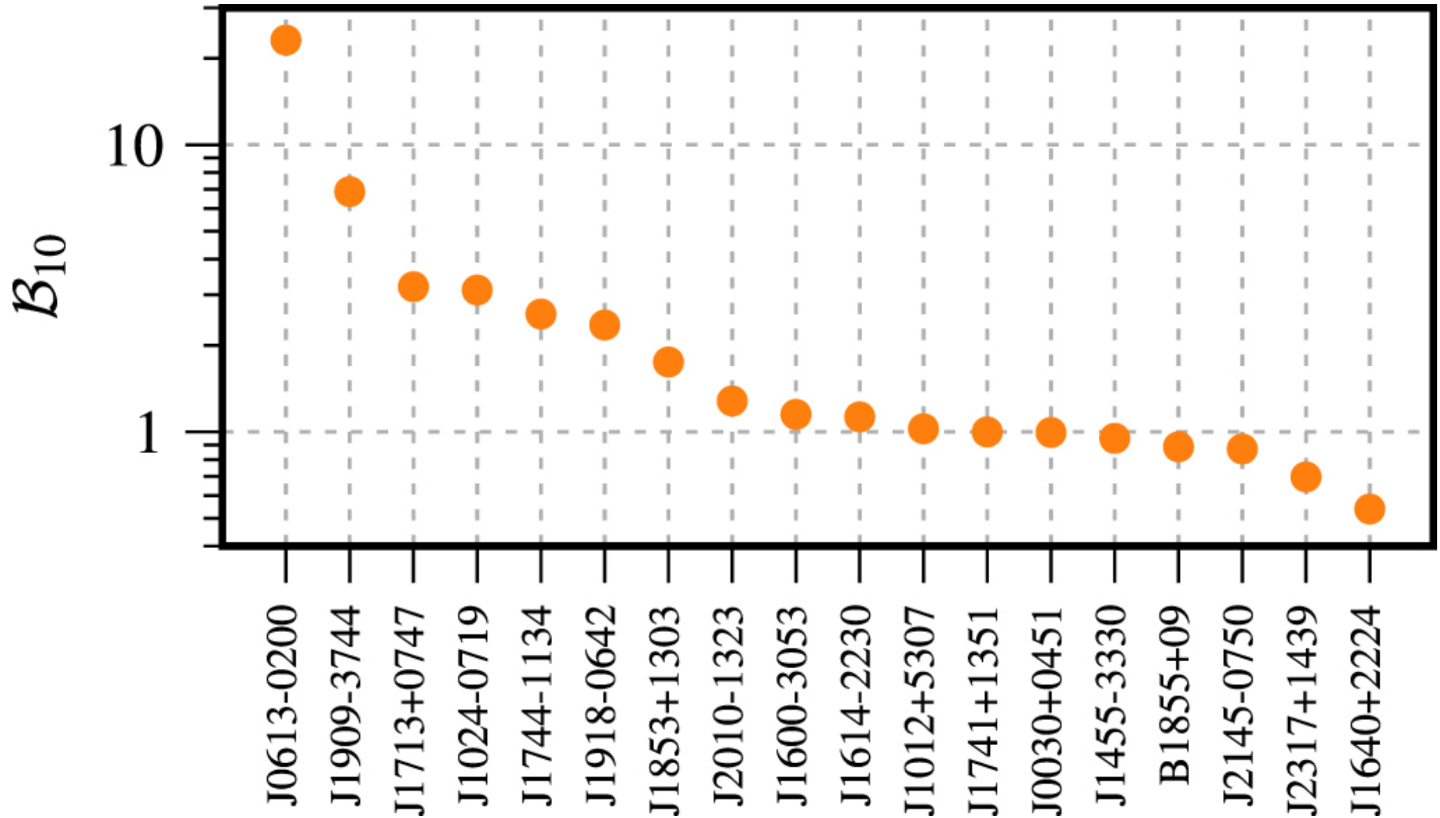
Figure 7. from The NANOGrav 11 yr Data Set: Limits on Gravitational Waves from Individual Supermassive Black Hole Binaries null 2019 APJ 880 116 doi:10.3847/1538-4357/ab2236 https://dx.doi.org/10.3847/1538-4357/ab2236 © 2019. The American Astronomical Society. All rights reserved.
