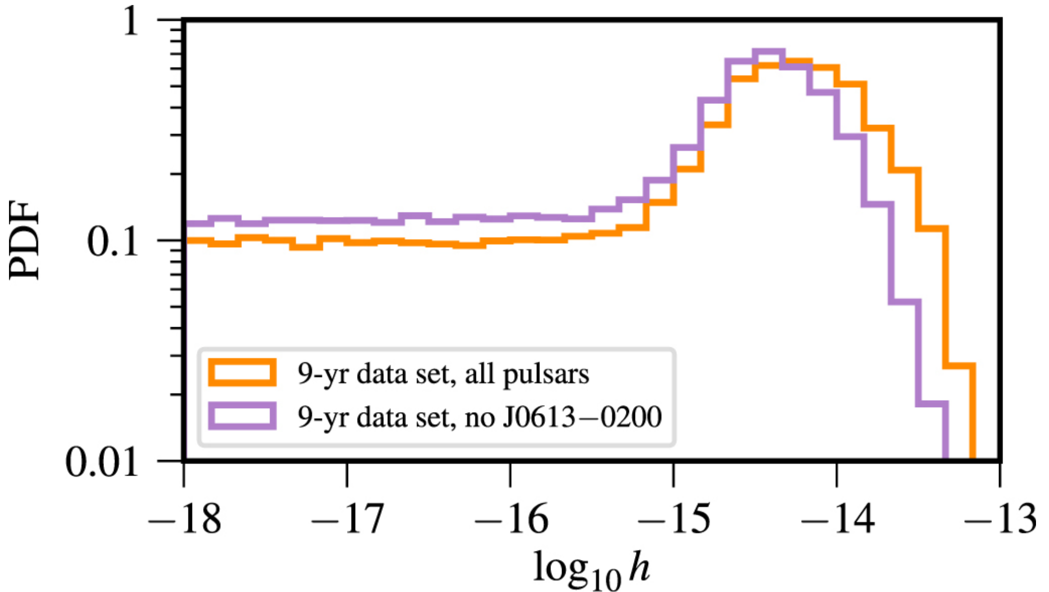
Figure 6. from The NANOGrav 11 yr Data Set: Limits on Gravitational Waves from Individual Supermassive Black Hole Binaries null 2019 APJ 880 116 doi:10.3847/1538-4357/ab2236 https://dx.doi.org/10.3847/1538-4357/ab2236 © 2019. The American Astronomical Society. All rights reserved.
