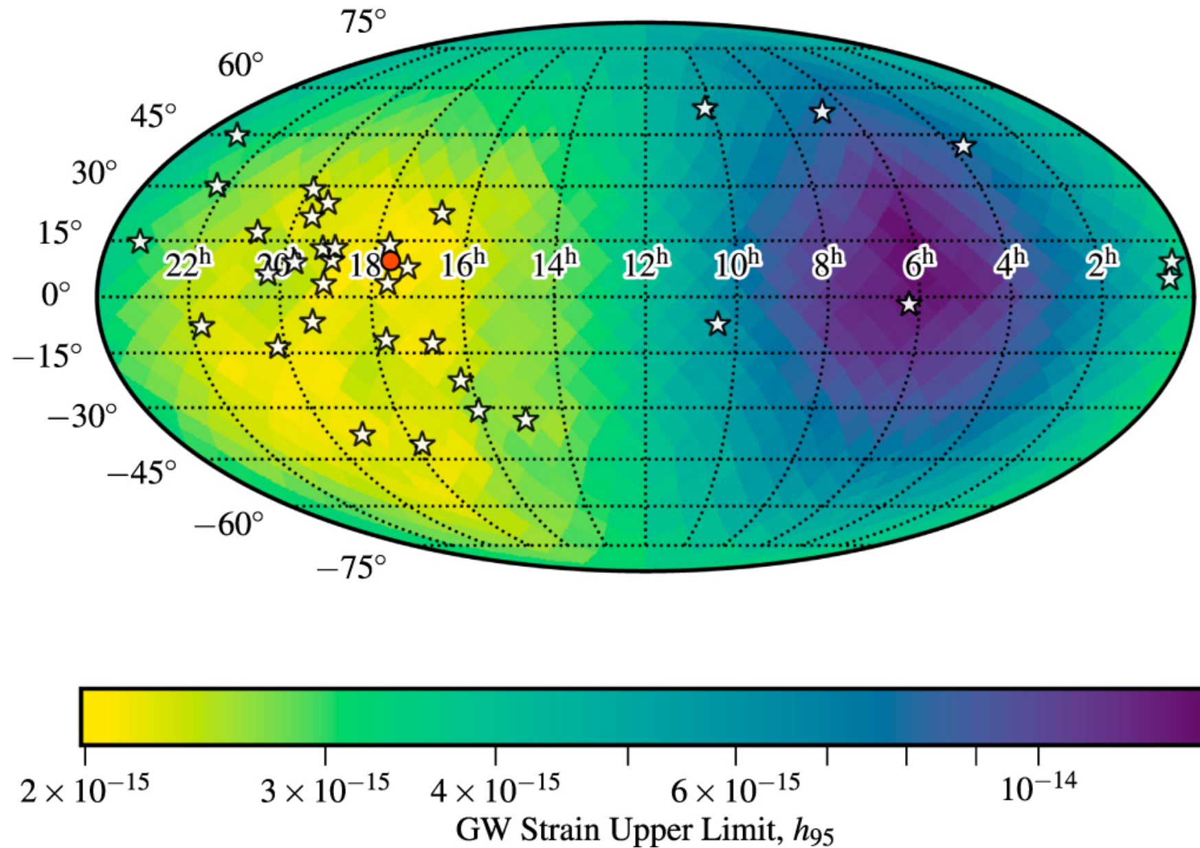
Figure 5. from The NANOGrav 11 yr Data Set: Limits on Gravitational Waves from Individual Supermassive Black Hole Binaries null 2019 APJ 880 116 doi:10.3847/1538-4357/ab2236 https://dx.doi.org/10.3847/1538-4357/ab2236 © 2019. The American Astronomical Society. All rights reserved.
