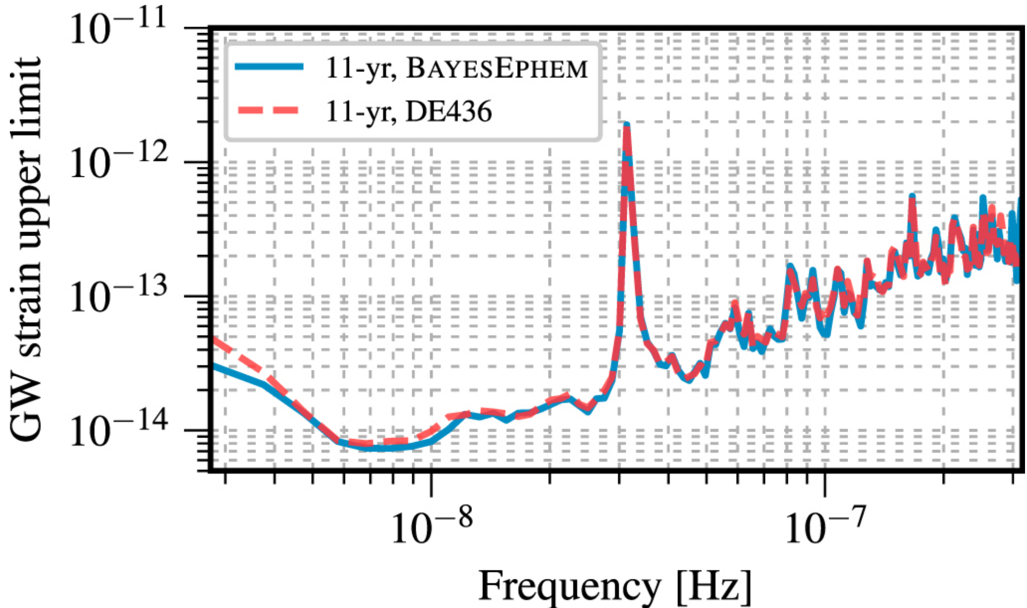
Figure 4. from The NANOGrav 11 yr Data Set: Limits on Gravitational Waves from Individual Supermassive Black Hole Binaries null 2019 APJ 880 116 doi:10.3847/1538-4357/ab2236 https://dx.doi.org/10.3847/1538-4357/ab2236 © 2019. The American Astronomical Society. All rights reserved.
