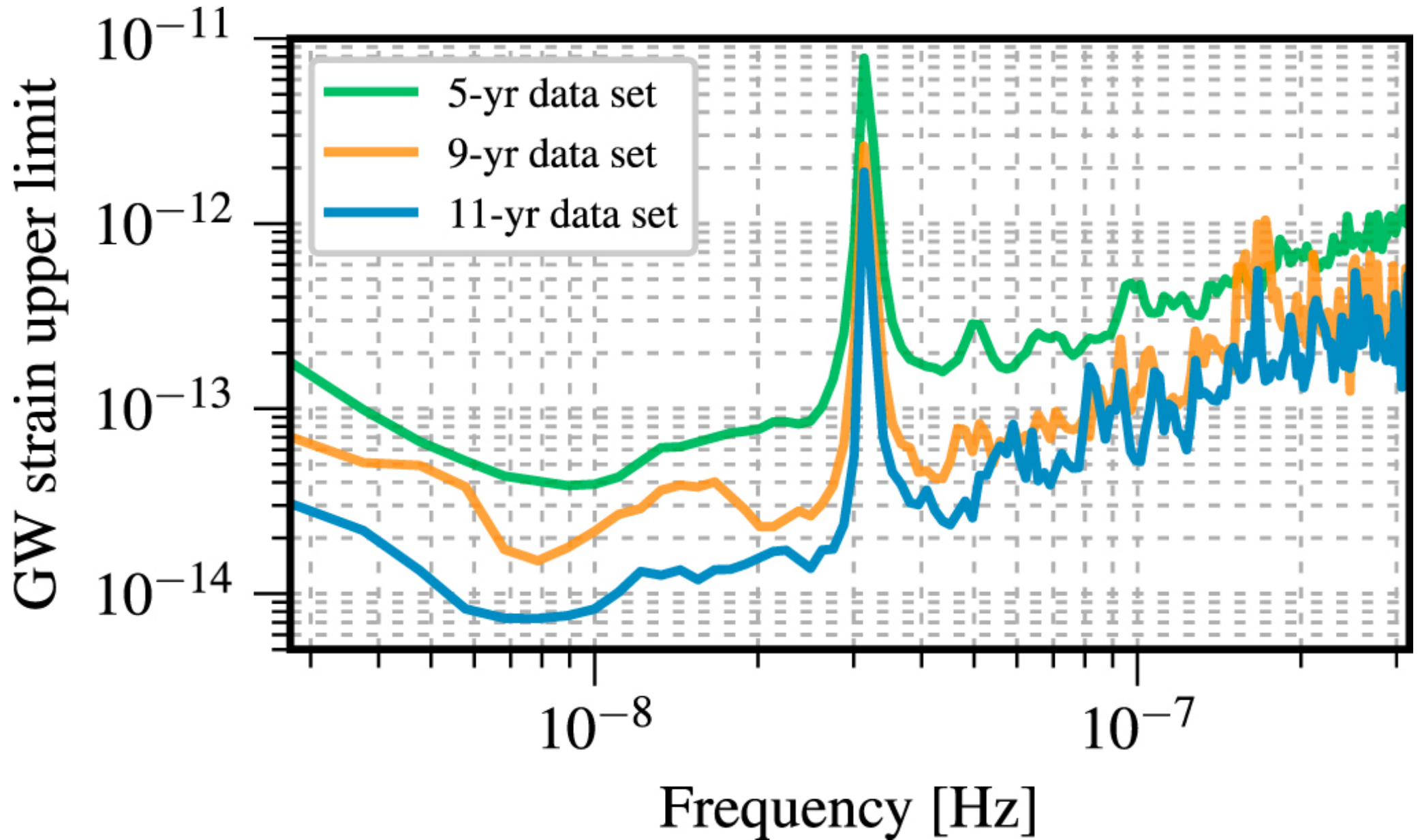
Figure 3. from The NANOGrav 11 yr Data Set: Limits on Gravitational Waves from Individual Supermassive Black Hole Binaries null 2019 APJ 880 116 doi:10.3847/1538-4357/ab2236 https://dx.doi.org/10.3847/1538-4357/ab2236 © 2019. The American Astronomical Society. All rights reserved.
