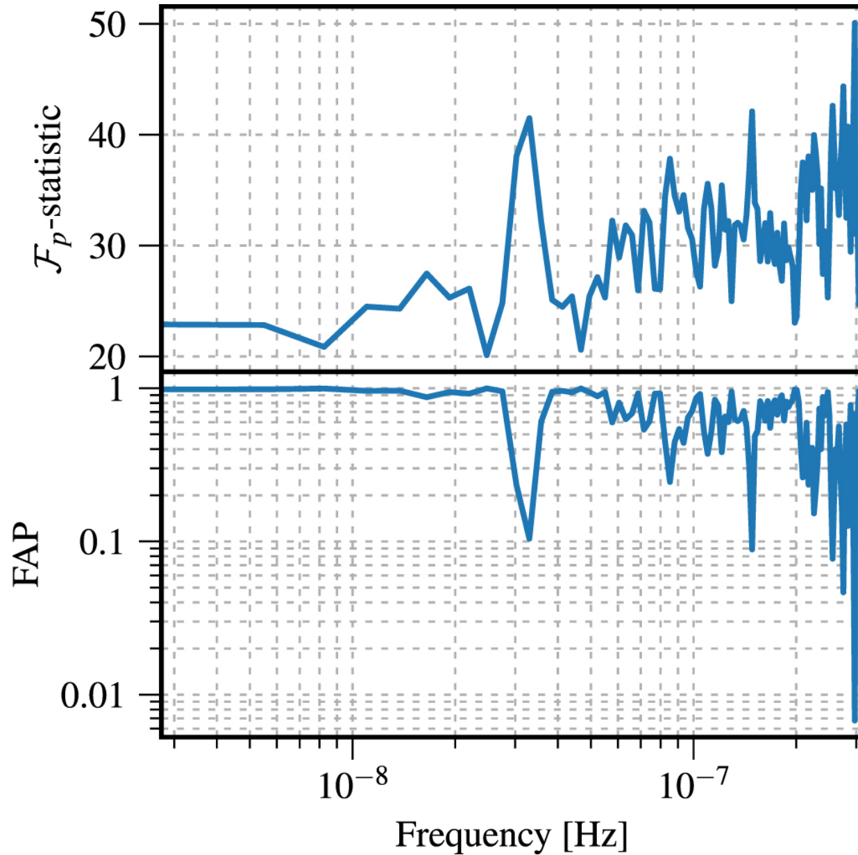
Figure 2. from The NANOGrav 11 yr Data Set: Limits on Gravitational Waves from Individual Supermassive Black Hole Binaries null 2019 APJ 880 116 doi:10.3847/1538-4357/ab2236 https://dx.doi.org/10.3847/1538-4357/ab2236 © 2019. The American Astronomical Society. All rights reserved.
