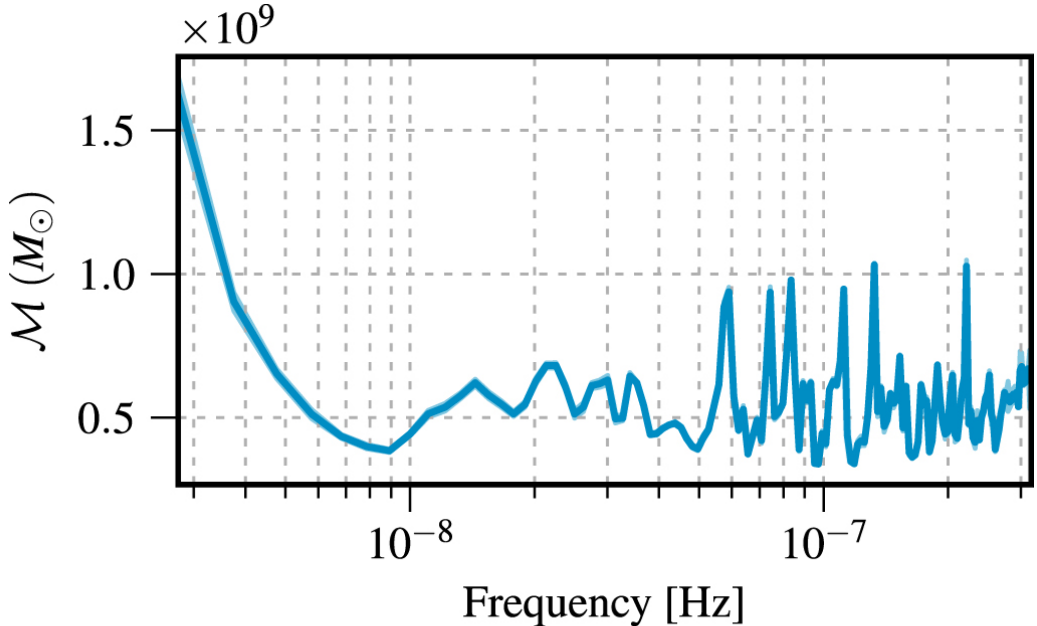
Figure 10. from The NANOGrav 11 yr Data Set: Limits on Gravitational Waves from Individual Supermassive Black Hole Binaries null 2019 APJ 880 116 doi:10.3847/1538-4357/ab2236 https://dx.doi.org/10.3847/1538-4357/ab2236 © 2019. The American Astronomical Society. All rights reserved.
