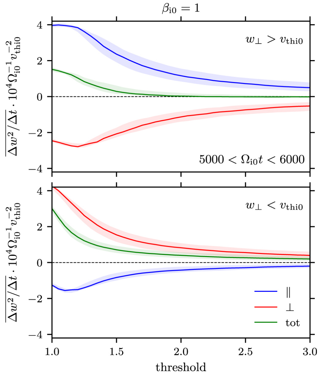
Figure 9. from Hybrid-kinetic Simulations of Ion Heating in Alfvénic Turbulence null 2019 APJ 879 53 doi:10.3847/1538-4357/ab20cc https://dx.doi.org/10.3847/1538-4357/ab20cc © 2019. The American Astronomical Society. All rights reserved.
