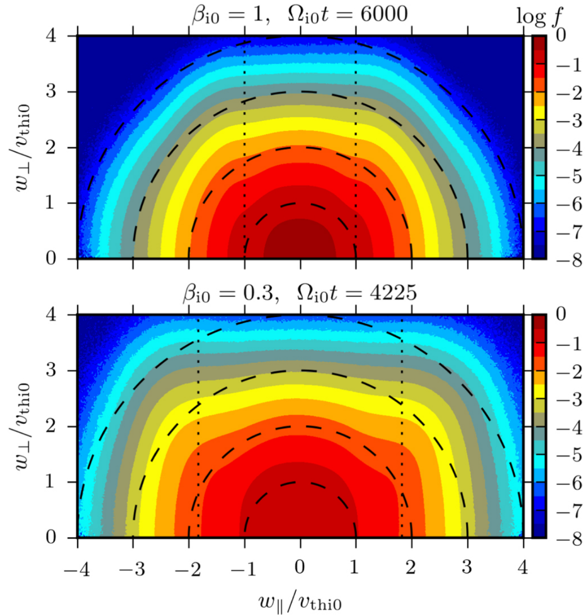
Figure 7. from Hybrid-kinetic Simulations of Ion Heating in Alfvénic Turbulence null 2019 APJ 879 53 doi:10.3847/1538-4357/ab20cc https://dx.doi.org/10.3847/1538-4357/ab20cc © 2019. The American Astronomical Society. All rights reserved.
