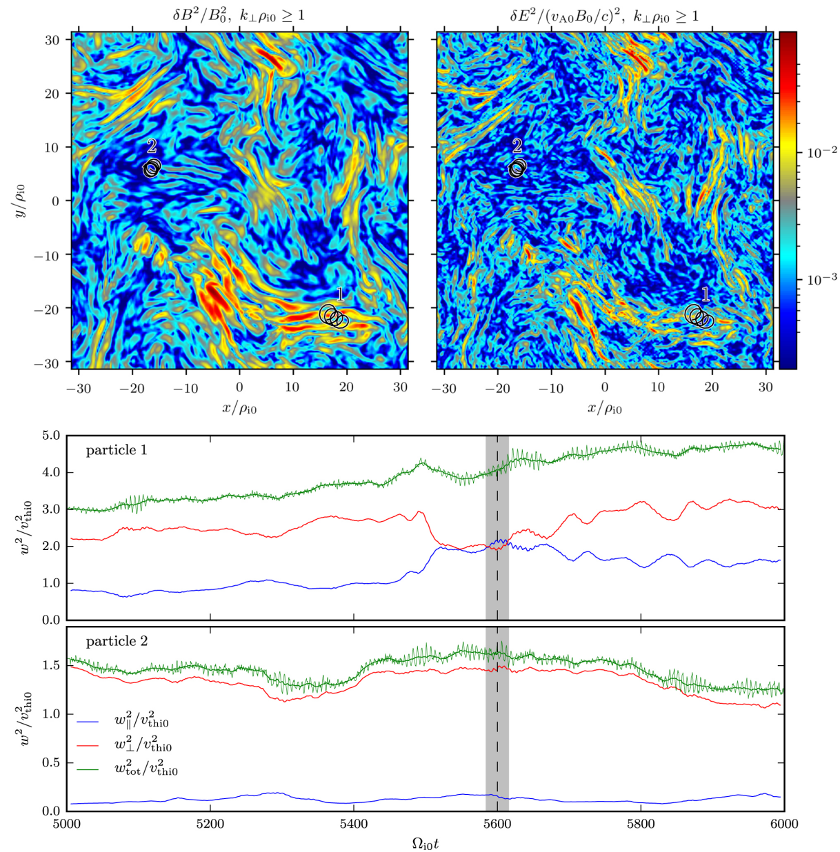
Figure 4. from Hybrid-kinetic Simulations of Ion Heating in Alfvénic Turbulence null 2019 APJ 879 53 doi:10.3847/1538-4357/ab20cc https://dx.doi.org/10.3847/1538-4357/ab20cc © 2019. The American Astronomical Society. All rights reserved.
