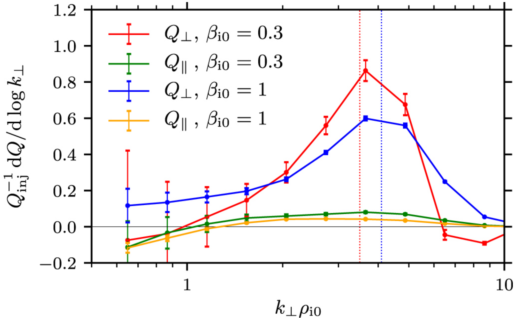
Figure 3. from Hybrid-kinetic Simulations of Ion Heating in Alfvénic Turbulence null 2019 APJ 879 53 doi:10.3847/1538-4357/ab20cc https://dx.doi.org/10.3847/1538-4357/ab20cc © 2019. The American Astronomical Society. All rights reserved.
