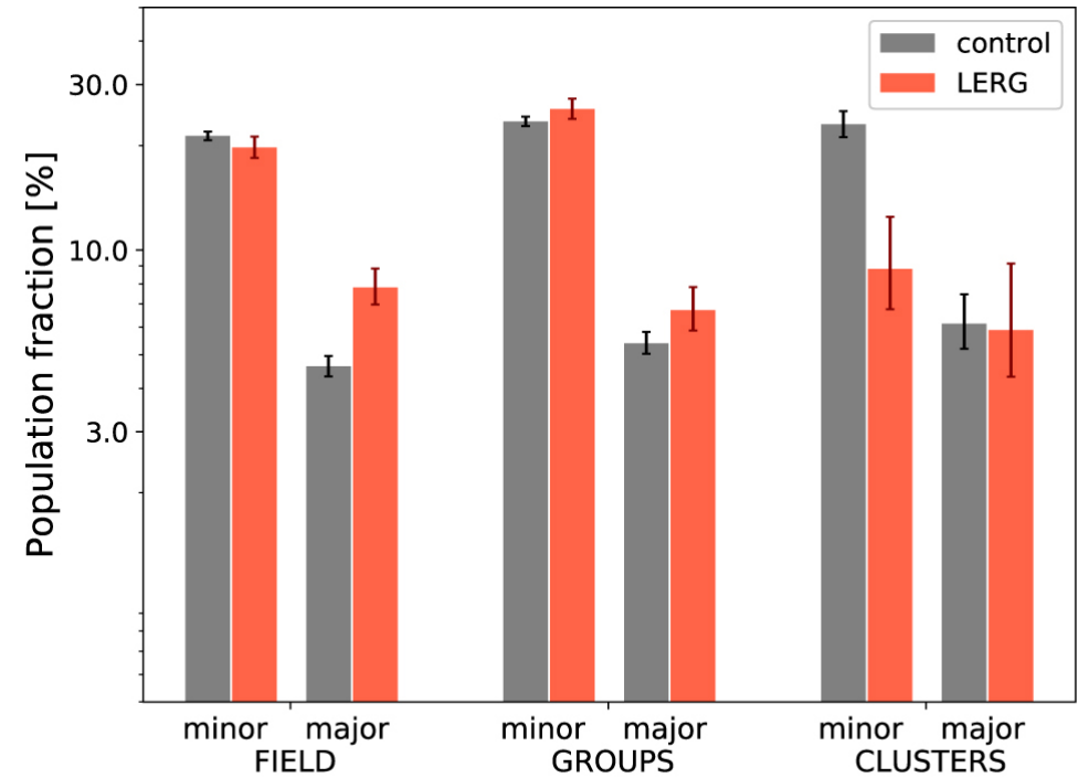
Figure 6. from The Effect of Minor and Major Mergers on the Evolution of Low-excitation Radio Galaxies null 2019 APJ 878 88 doi:10.3847/1538-4357/ab203f https://dx.doi.org/10.3847/1538-4357/ab203f © 2019. The American Astronomical Society. All rights reserved.
