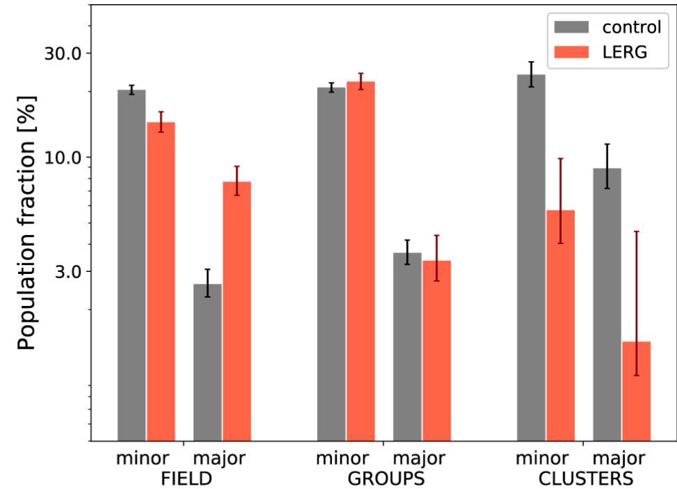
Figure 6. from The Effect of Minor and Major Mergers on the Evolution of Low-excitation Radio Galaxies null 2019 APJ 878 88 doi:10.3847/1538-4357/ab203f https://dx.doi.org/10.3847/1538-4357/ab203f © 2019. The American Astronomical Society. All rights reserved.
