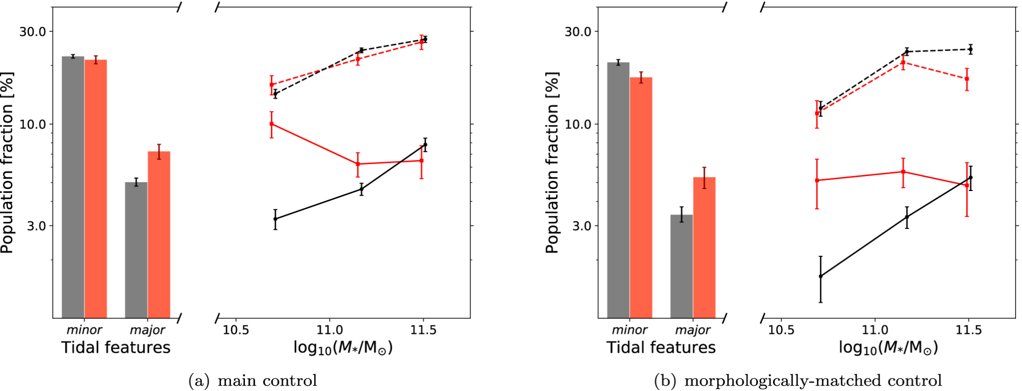
Figure 5. from The Effect of Minor and Major Mergers on the Evolution of Low-excitation Radio Galaxies null 2019 APJ 878 88 doi:10.3847/1538-4357/ab203f https://dx.doi.org/10.3847/1538-4357/ab203f © 2019. The American Astronomical Society. All rights reserved.
