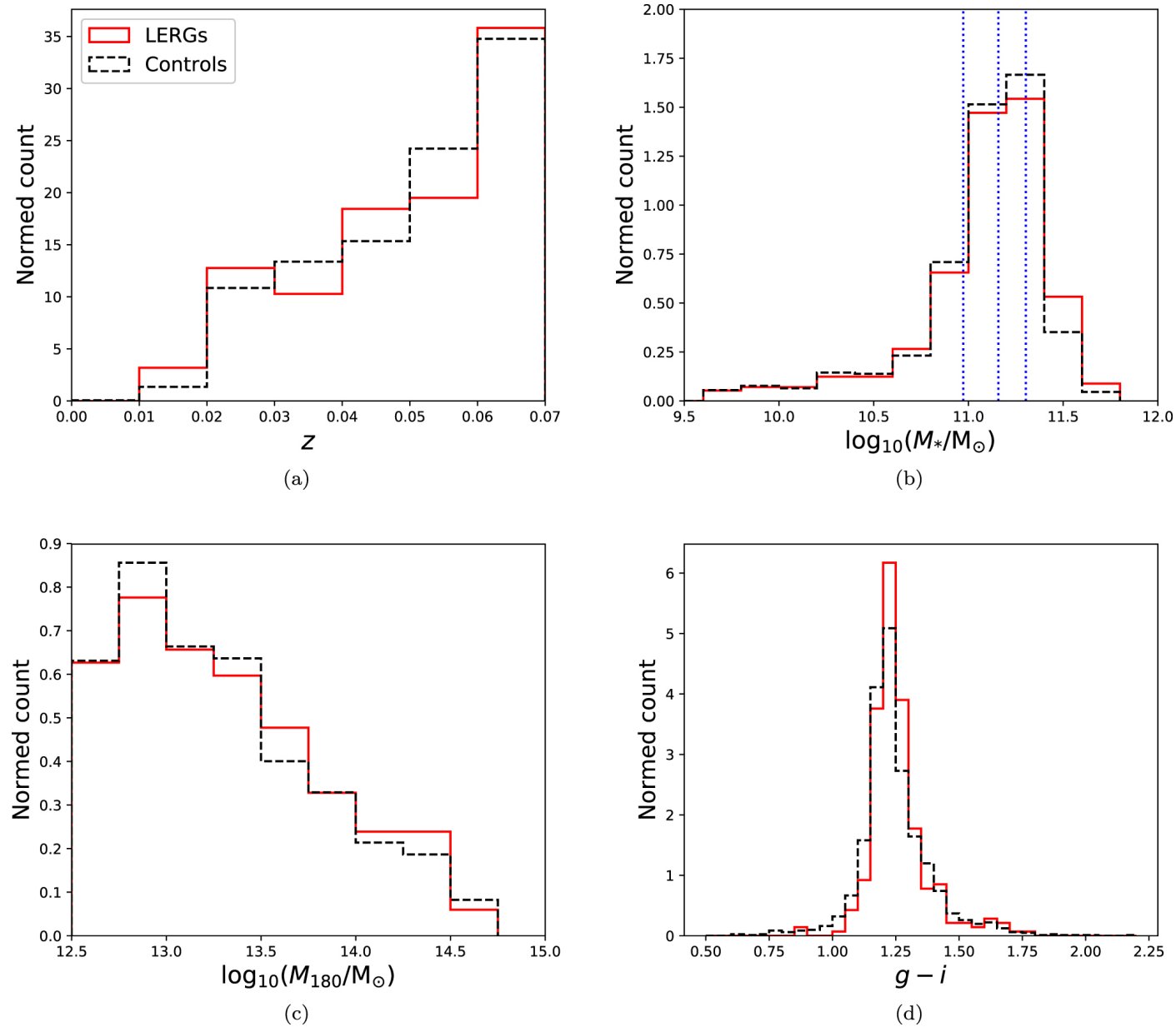
Figure 3. from The Effect of Minor and Major Mergers on the Evolution of Low-excitation Radio Galaxies null 2019 APJ 878 88 doi:10.3847/1538-4357/ab203f https://dx.doi.org/10.3847/1538-4357/ab203f © 2019. The American Astronomical Society. All rights reserved.
