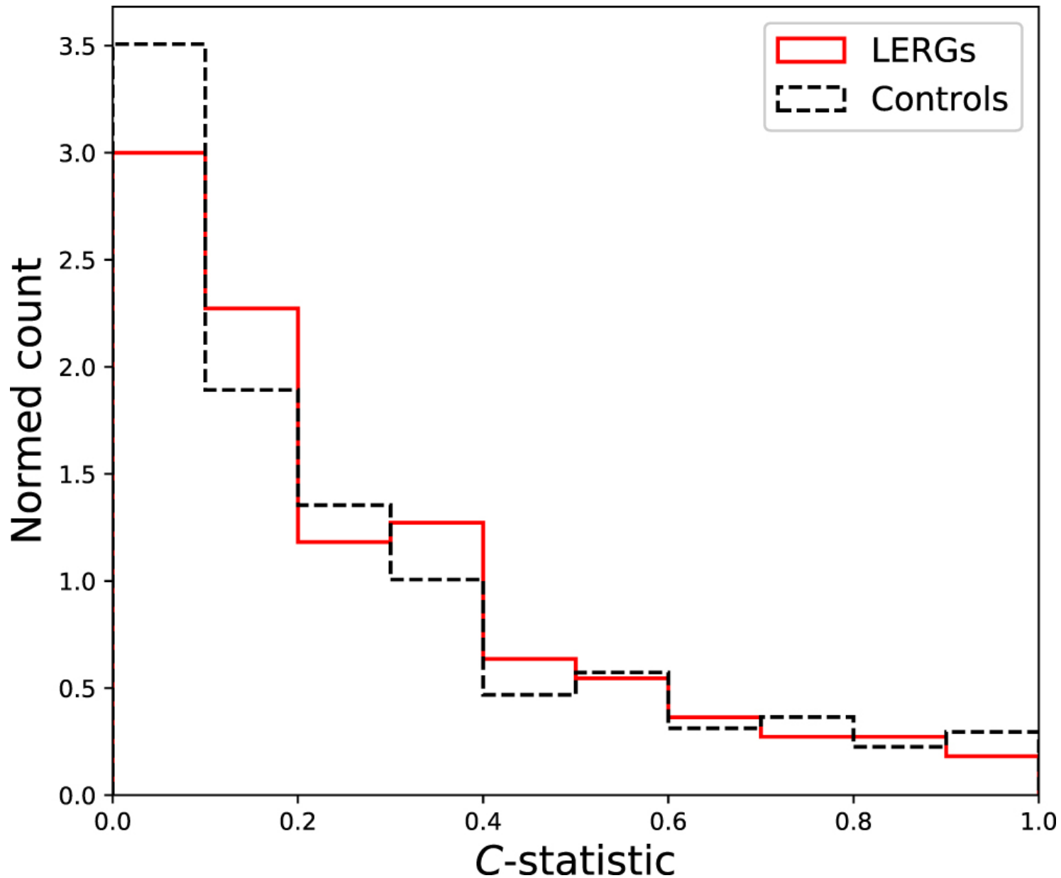
Figure 2. from The Effect of Minor and Major Mergers on the Evolution of Low-excitation Radio Galaxies null 2019 APJ 878 88 doi:10.3847/1538-4357/ab203f https://dx.doi.org/10.3847/1538-4357/ab203f © 2019. The American Astronomical Society. All rights reserved.
