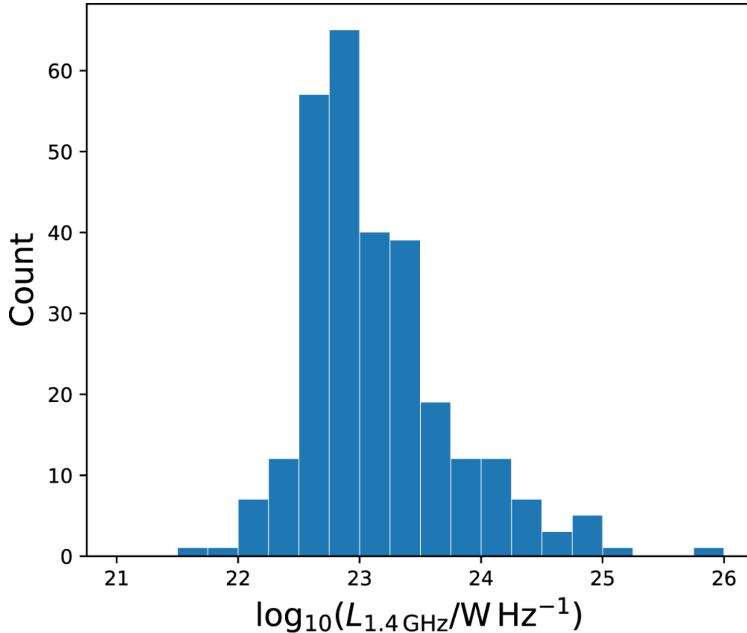
Figure 1. from The Effect of Minor and Major Mergers on the Evolution of Low-excitation Radio Galaxies null 2019 APJ 878 88 doi:10.3847/1538-4357/ab203f https://dx.doi.org/10.3847/1538-4357/ab203f © 2019. The American Astronomical Society. All rights reserved.
