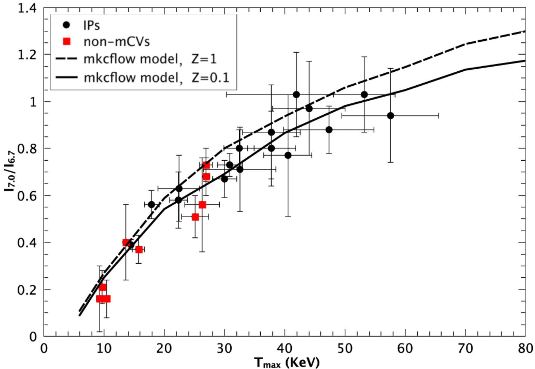
Figure 2. from The Fe Line Flux Ratio as a Diagnostic of the Maximum Temperature and the White Dwarf Mass of Cataclysmic Variables null 2019 APJ 878 53 doi:10.3847/1538-4357/ab1fe1 https://dx.doi.org/10.3847/1538-4357/ab1fe1 © 2019. The American Astronomical Society.
