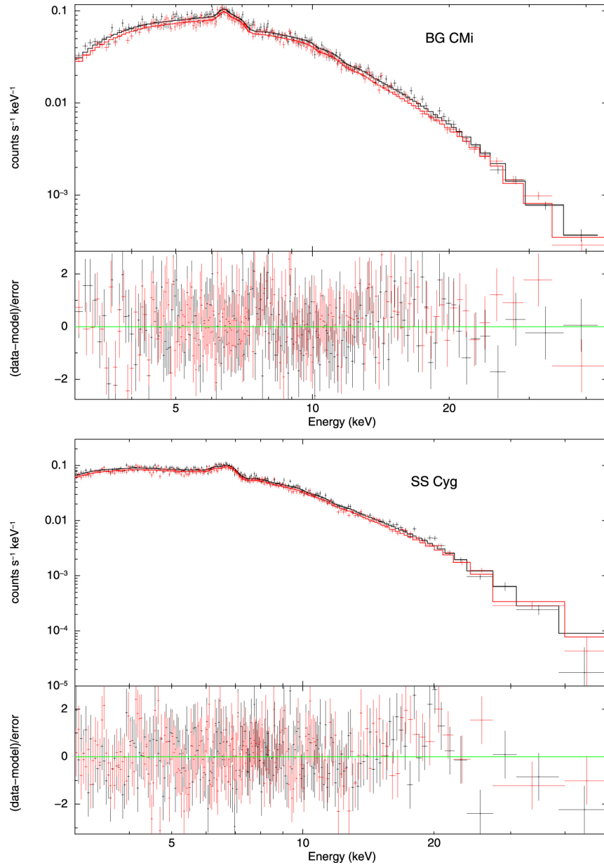
Figure 1. from The Fe Line Flux Ratio as a Diagnostic of the Maximum Temperature and the White Dwarf Mass of Cataclysmic Variables null 2019 APJ 878 53 doi:10.3847/1538-4357/ab1fe1 https://dx.doi.org/10.3847/1538-4357/ab1fe1 © 2019. The American Astronomical Society.
