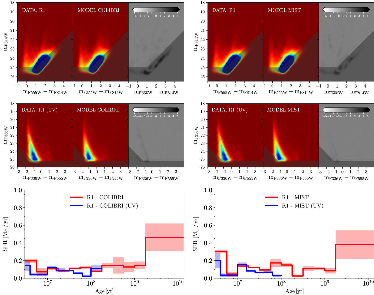
Figure 9. from Star Formation Histories of the LEGUS Spiral Galaxies. I. The Flocculent Spiral NGC 7793 null 2019 APJ 878 1 doi:10.3847/1538-4357/ab1de1 https://dx.doi.org/10.3847/1538-4357/ab1de1
