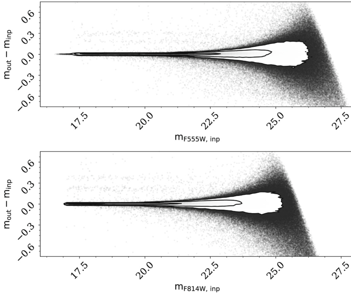
Figure 7. from Star Formation Histories of the LEGUS Spiral Galaxies. I. The Flocculent Spiral NGC 7793 null 2019 APJ 878 1 doi:10.3847/1538-4357/ab1de1 https://dx.doi.org/10.3847/1538-4357/ab1de1 © 2019. The American Astronomical Society. All rights reserved.
