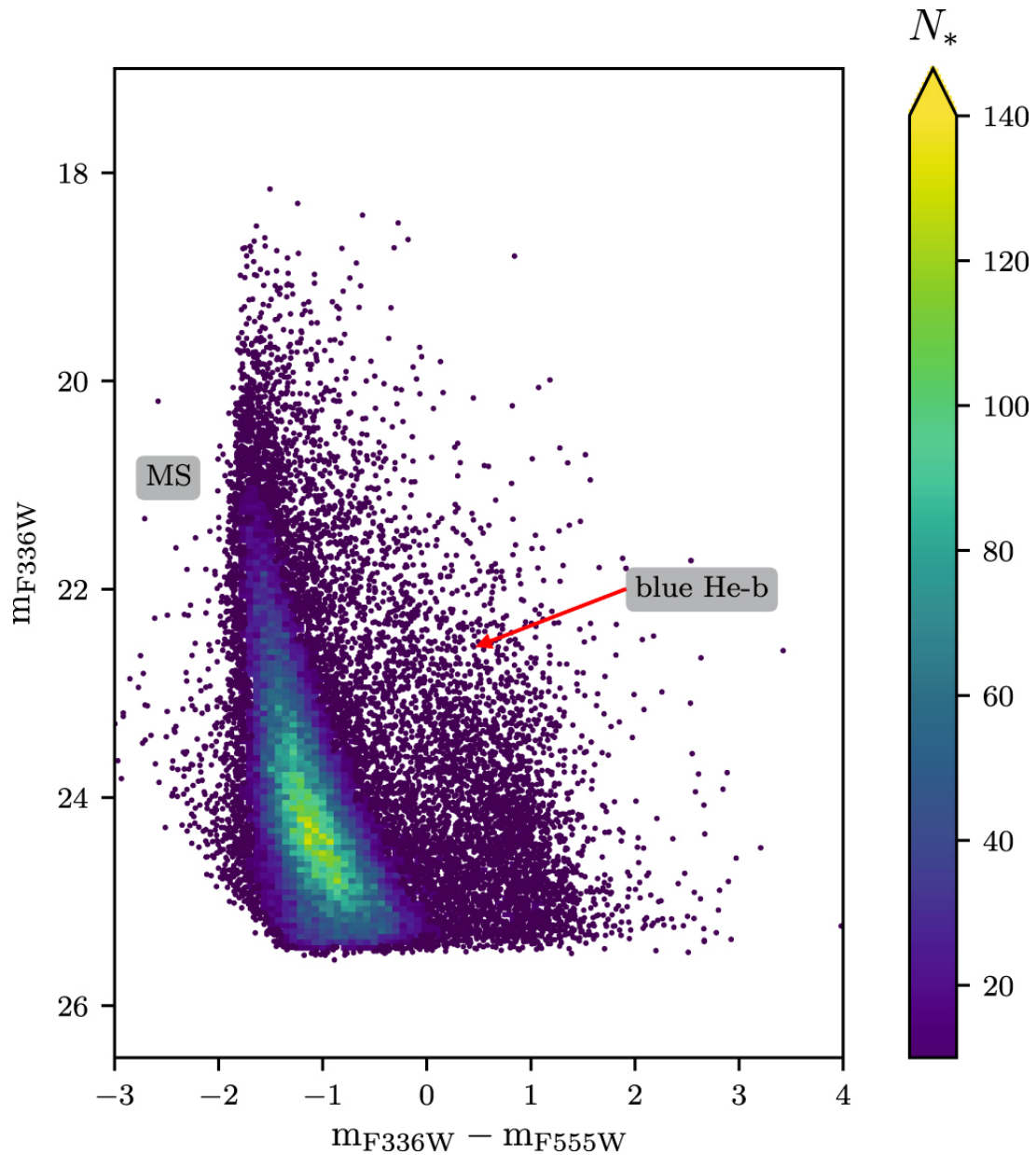
Figure 3. from Star Formation Histories of the LEGUS Spiral Galaxies. I. The Flocculent Spiral NGC 7793 null 2019 APJ 878 1 doi:10.3847/1538-4357/ab1de1 https://dx.doi.org/10.3847/1538-4357/ab1de1 © 2019. The American Astronomical Society. All rights reserved.
