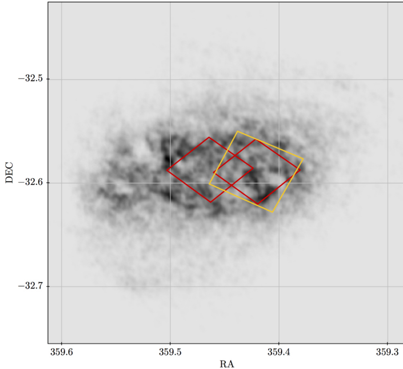
Figure 14. from Star Formation Histories of the LEGUS Spiral Galaxies. I. The Flocculent Spiral NGC 7793 null 2019 APJ 878 1 doi:10.3847/1538-4357/ab1de1 https://dx.doi.org/10.3847/1538-4357/ab1de1 © 2019. The American Astronomical Society. All rights reserved.
