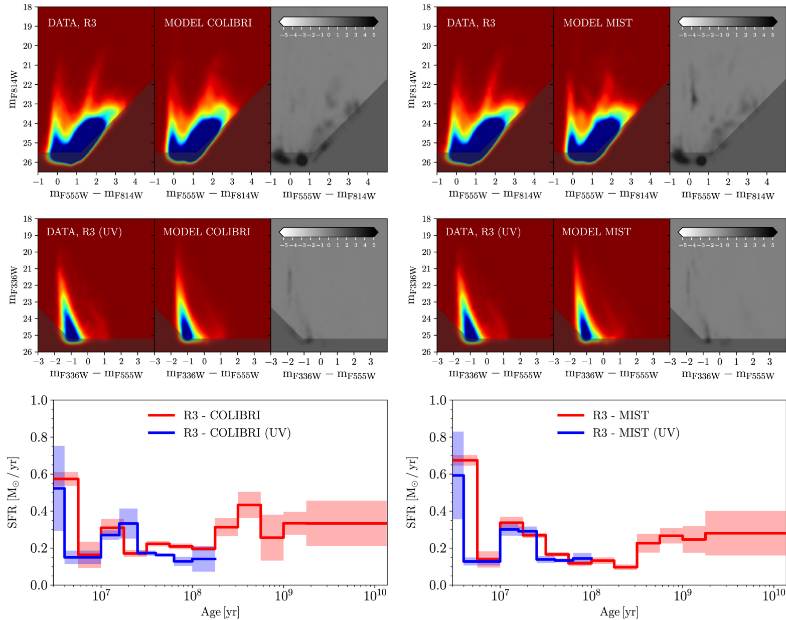
Figure 11. from Star Formation Histories of the LEGUS Spiral Galaxies. I. The Flocculent Spiral NGC 7793 null 2019 APJ 878 1 doi:10.3847/1538-4357/ab1de1 https://dx.doi.org/10.3847/1538-4357/ab1de1
