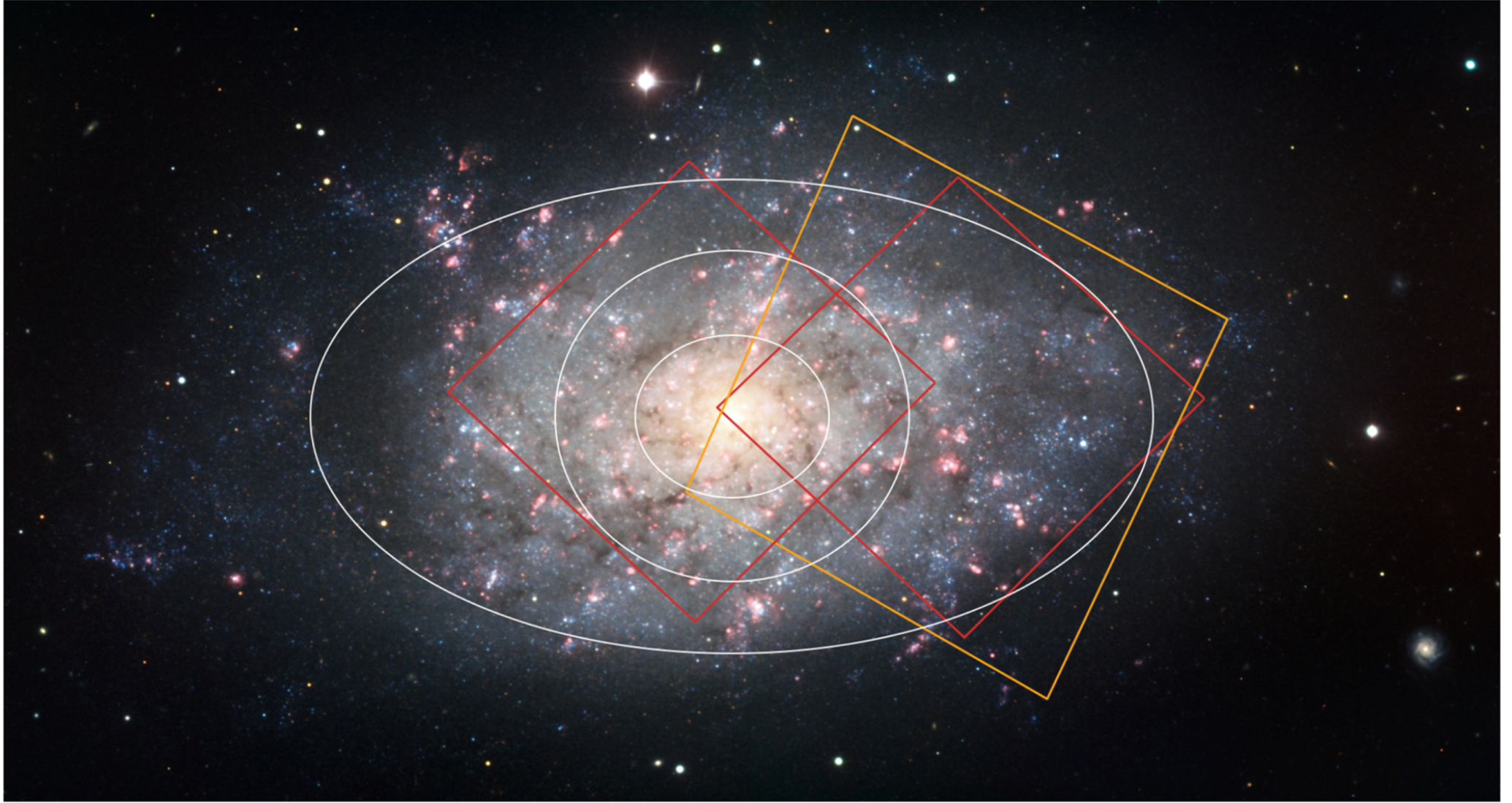
Figure 1. from Star Formation Histories of the LEGUS Spiral Galaxies. I. The Flocculent Spiral NGC 7793 null 2019 APJ 878 1 doi:10.3847/1538-4357/ab1de1 https://dx.doi.org/10.3847/1538-4357/ab1de1 © 2019. The American Astronomical Society. All rights reserved.
