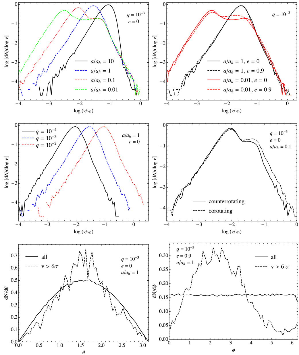
Figure 4. from Hypervelocity Stars from a Supermassive Black Hole–Intermediate-mass Black Hole Binary null 2019 APJ 878 17 doi:10.3847/1538-4357/ab1c5d https://dx.doi.org/10.3847/1538-4357/ab1c5d © 2019. The American Astronomical Society. All rights reserved.
