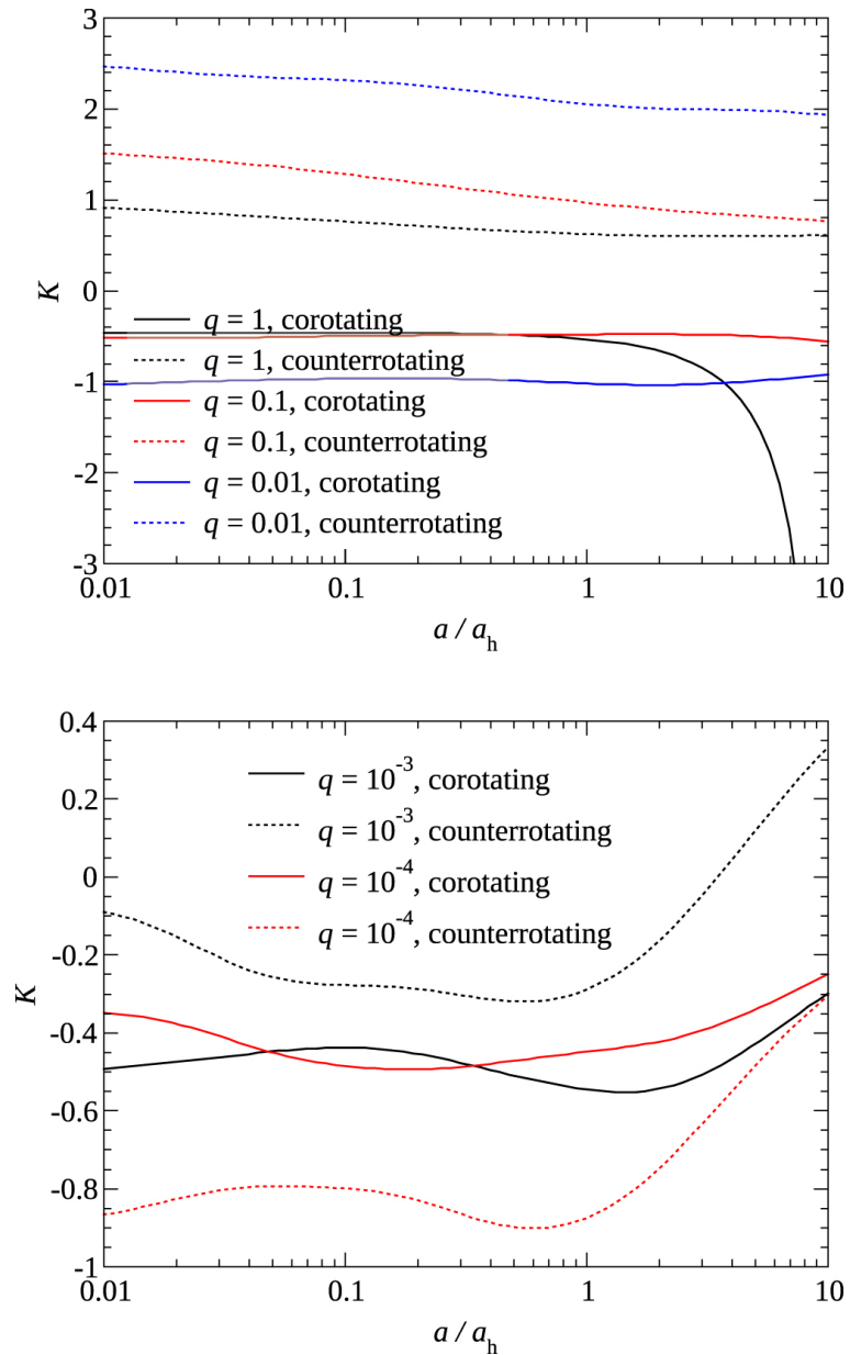
Figure 3. from Hypervelocity Stars from a Supermassive Black Hole–Intermediate-mass Black Hole Binary null 2019 APJ 878 17 doi:10.3847/1538-4357/ab1c5d https://dx.doi.org/10.3847/1538-4357/ab1c5d
