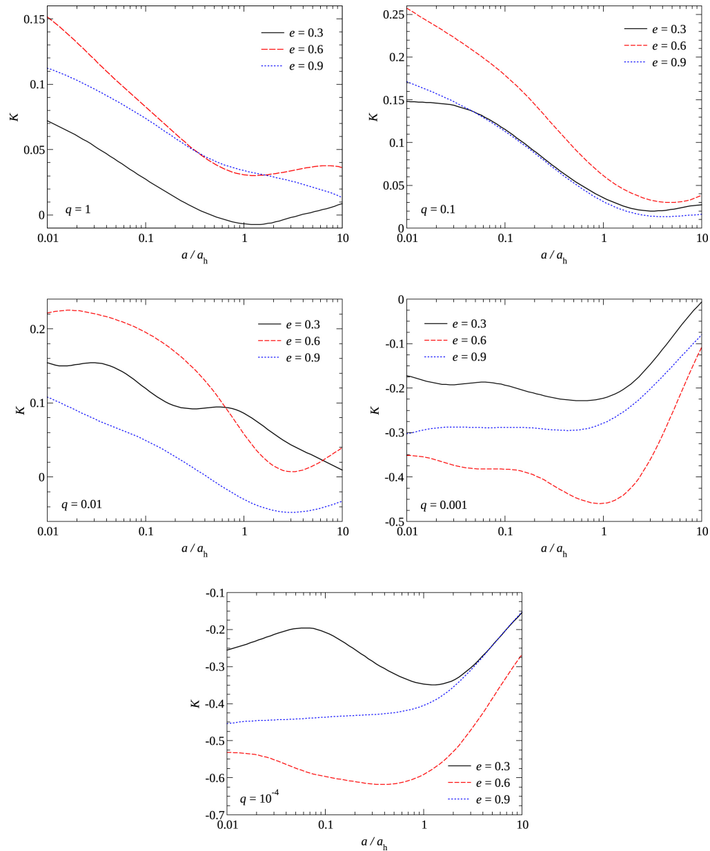
Figure 2. from Hypervelocity Stars from a Supermassive Black Hole–Intermediate-mass Black Hole Binary null 2019 APJ 878 17 doi:10.3847/1538-4357/ab1c5d https://dx.doi.org/10.3847/1538-4357/ab1c5d © 2019. The American Astronomical Society. All rights reserved.
