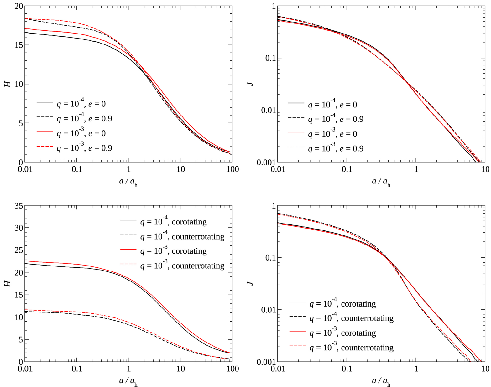
Figure 1. from Hypervelocity Stars from a Supermassive Black Hole–Intermediate-mass Black Hole Binary null 2019 APJ 878 17 doi:10.3847/1538-4357/ab1c5d https://dx.doi.org/10.3847/1538-4357/ab1c5d
