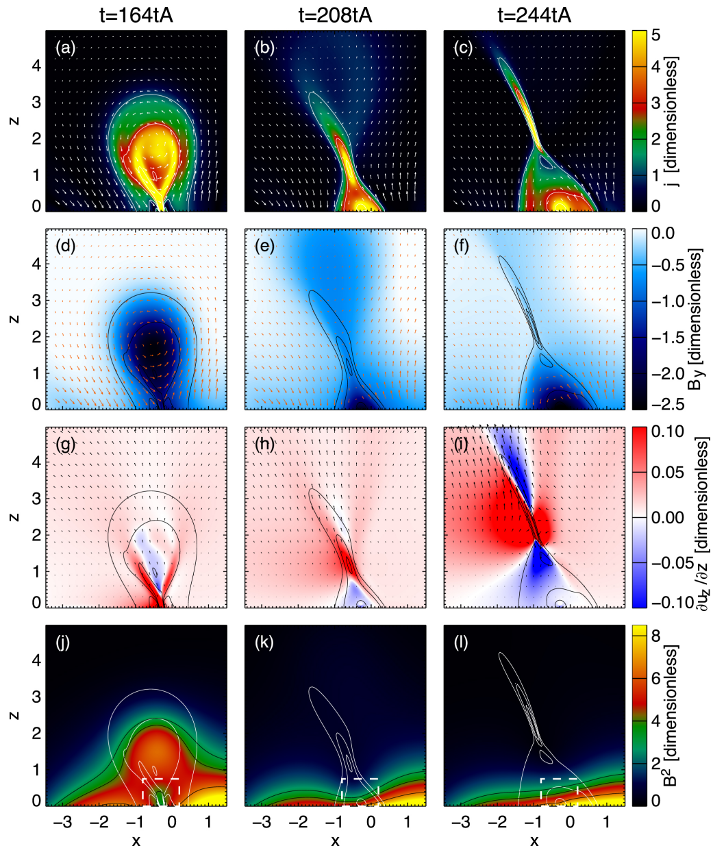
Figure 11. from Flare Reconnection-driven Magnetic Field and Lorentz Force Variations at the Sun's Surface null 2019 APJ 877 67 doi:10.3847/1538-4357/ab1b3d https://dx.doi.org/10.3847/1538-4357/ab1b3d
