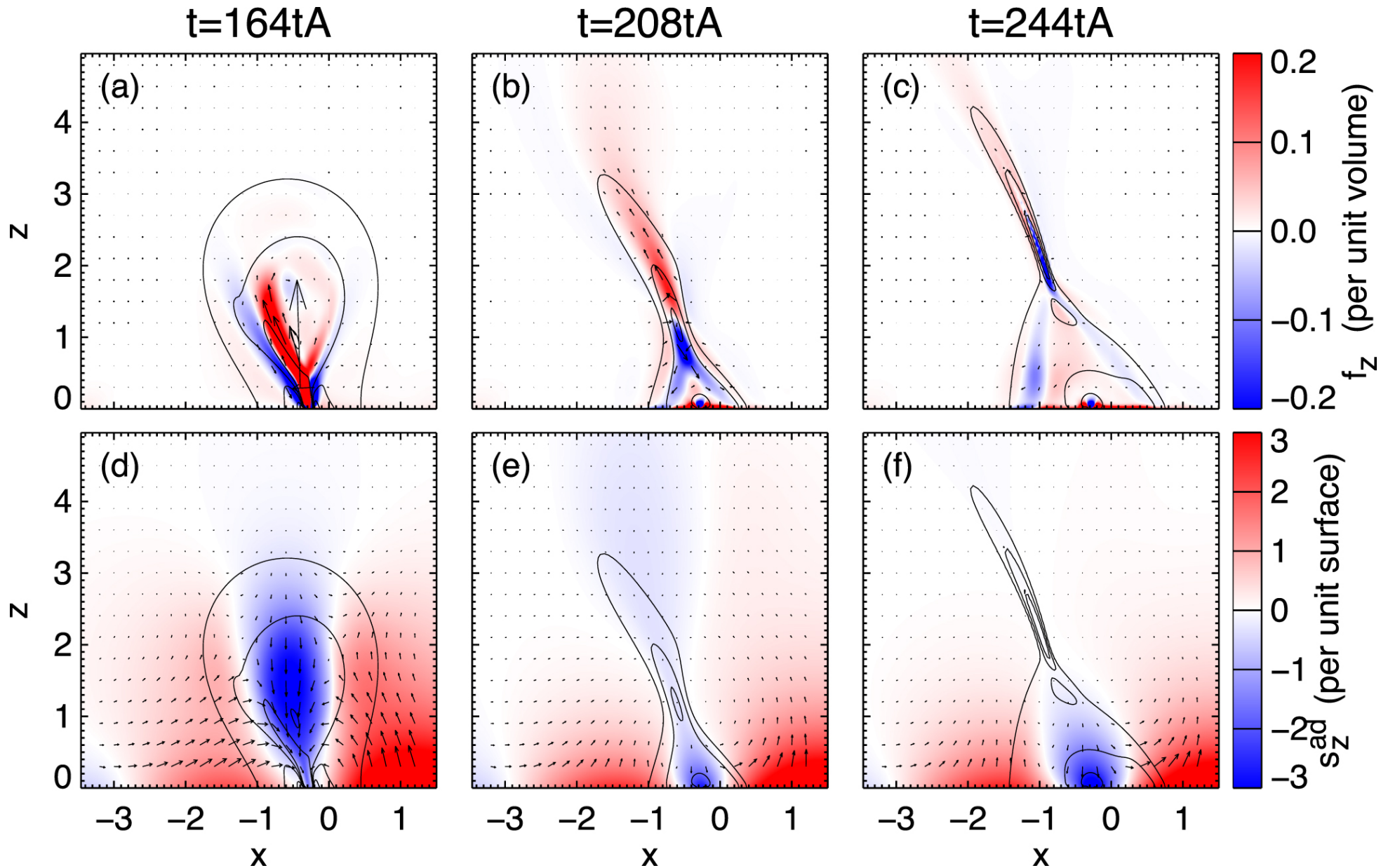
Figure 10. from Flare Reconnection-driven Magnetic Field and Lorentz Force Variations at the Sun's Surface null 2019 APJ 877 67 doi:10.3847/1538-4357/ab1b3d https://dx.doi.org/10.3847/1538-4357/ab1b3d © 2019. The American Astronomical Society. All rights reserved.
